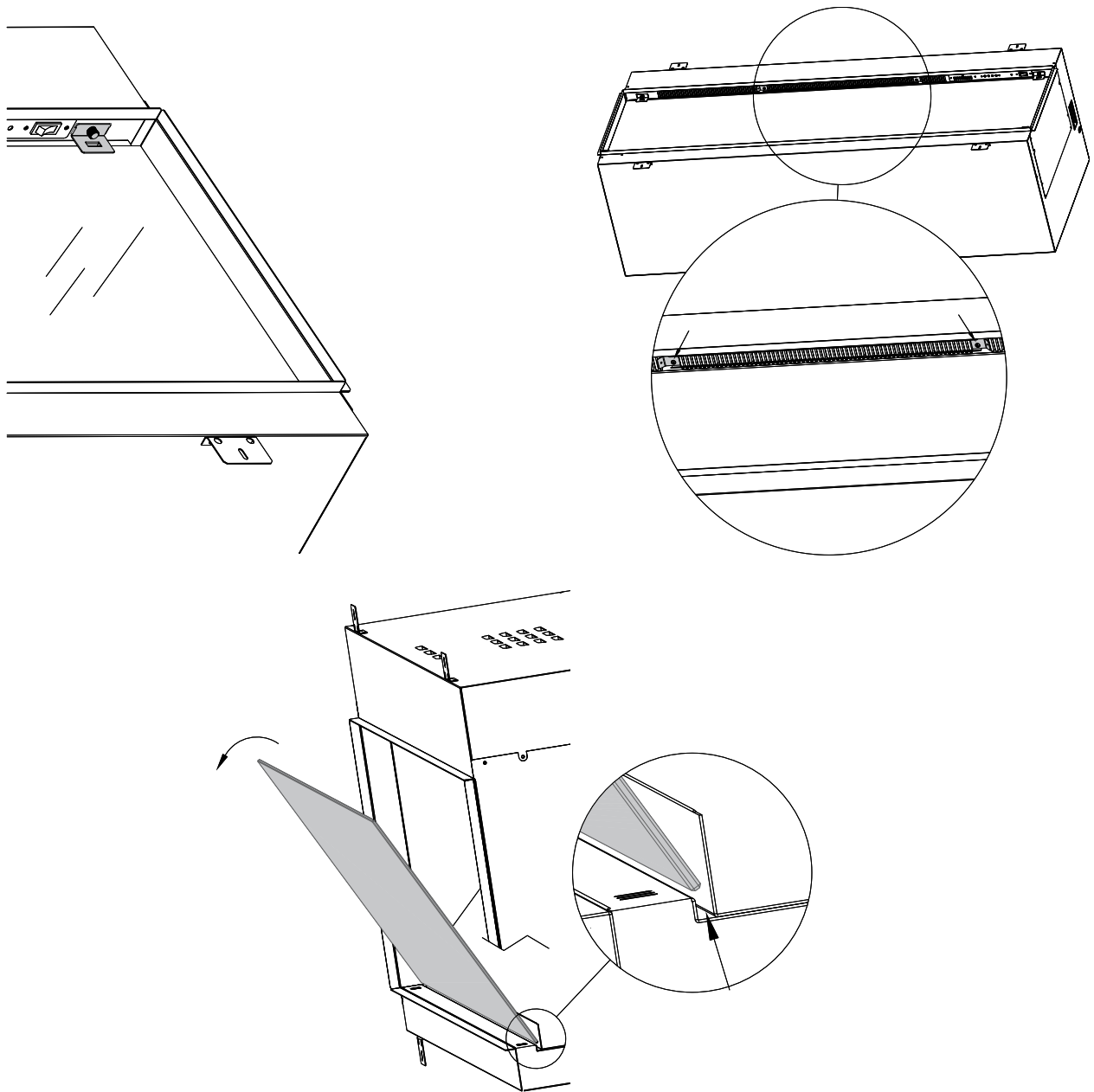
Figure 4.1 - Glass Removal
