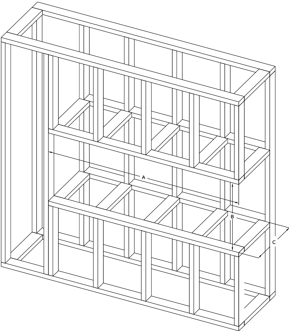
Figure 2.7 - Framed Opening - Corner Installation
