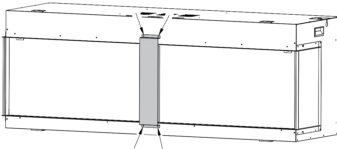
Figure 2.2 - Shipping Brace
