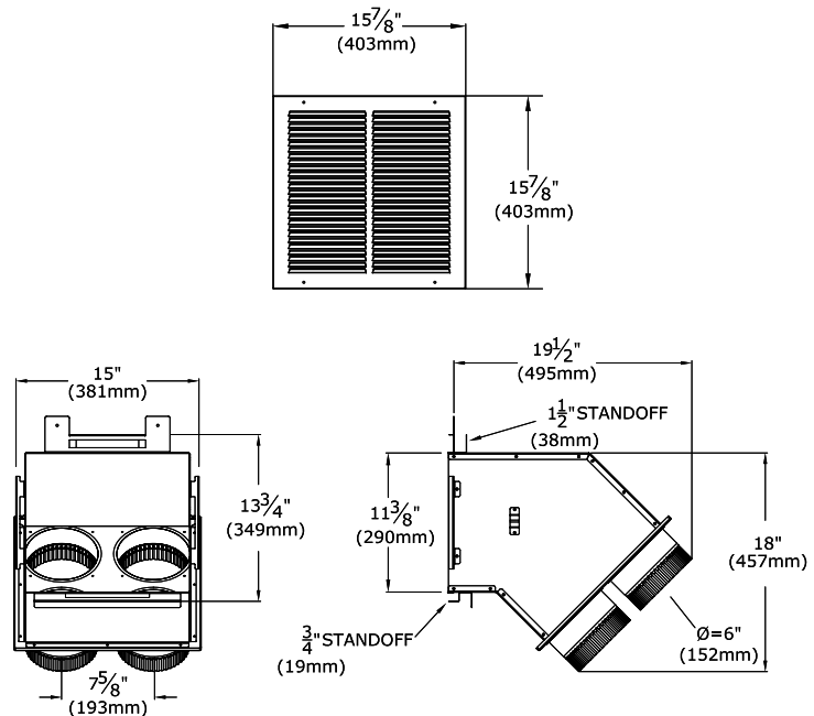
Figure 3.11 - KZK-1616 Overview
