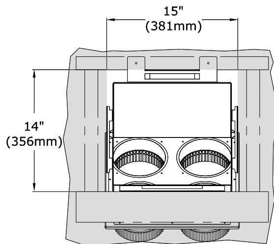
Figure 3.14 - Finishing Side KZK Plenum Opening
