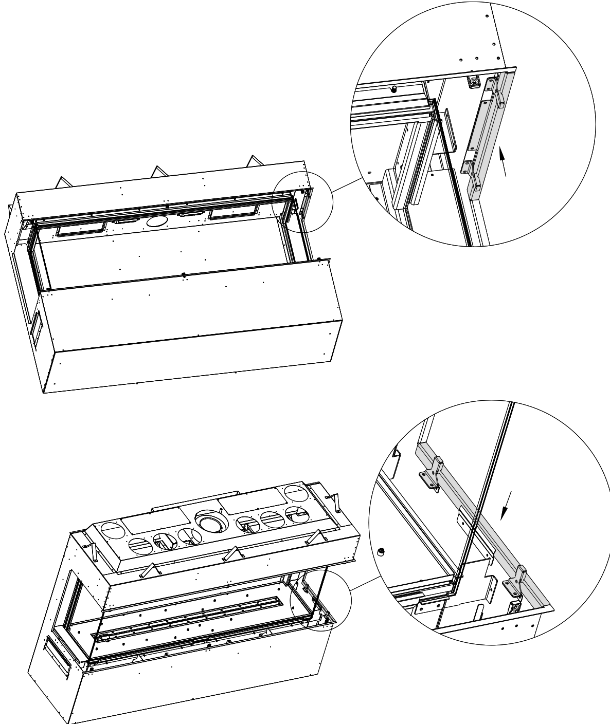
Figure 1.2 - Fireplace Conversion
