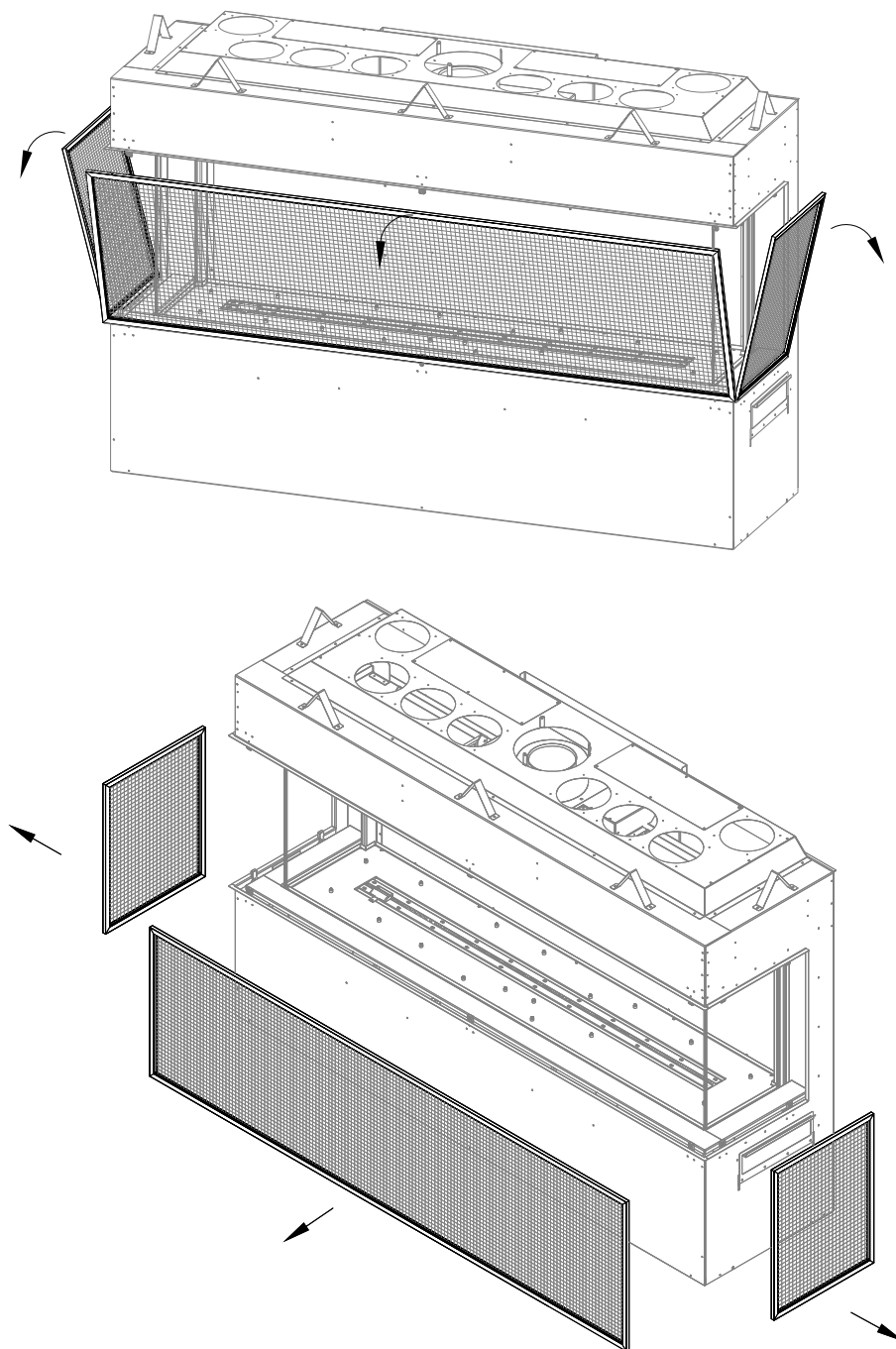
Figure 4.2 - Safety Screen Removal
