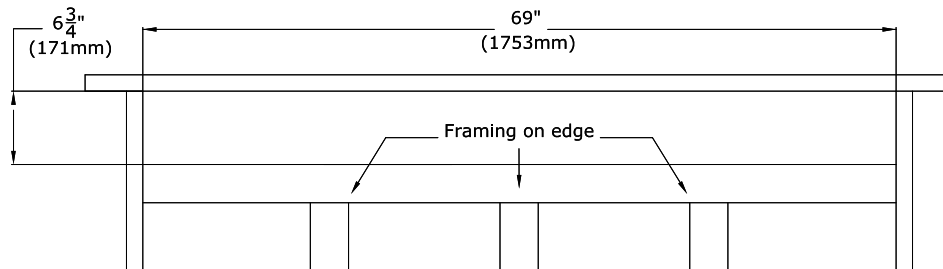
Figure 2.7 - Front KZK - Plenum Framed Opening
