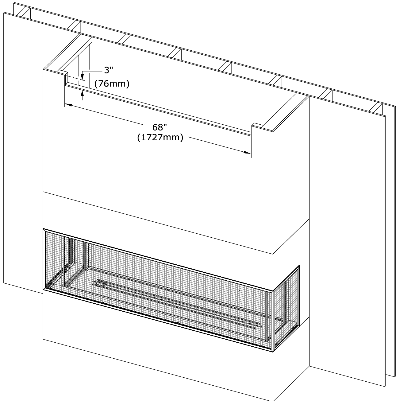
Figure 3.19 - Air Opening - Front Facing Vented Cavity
