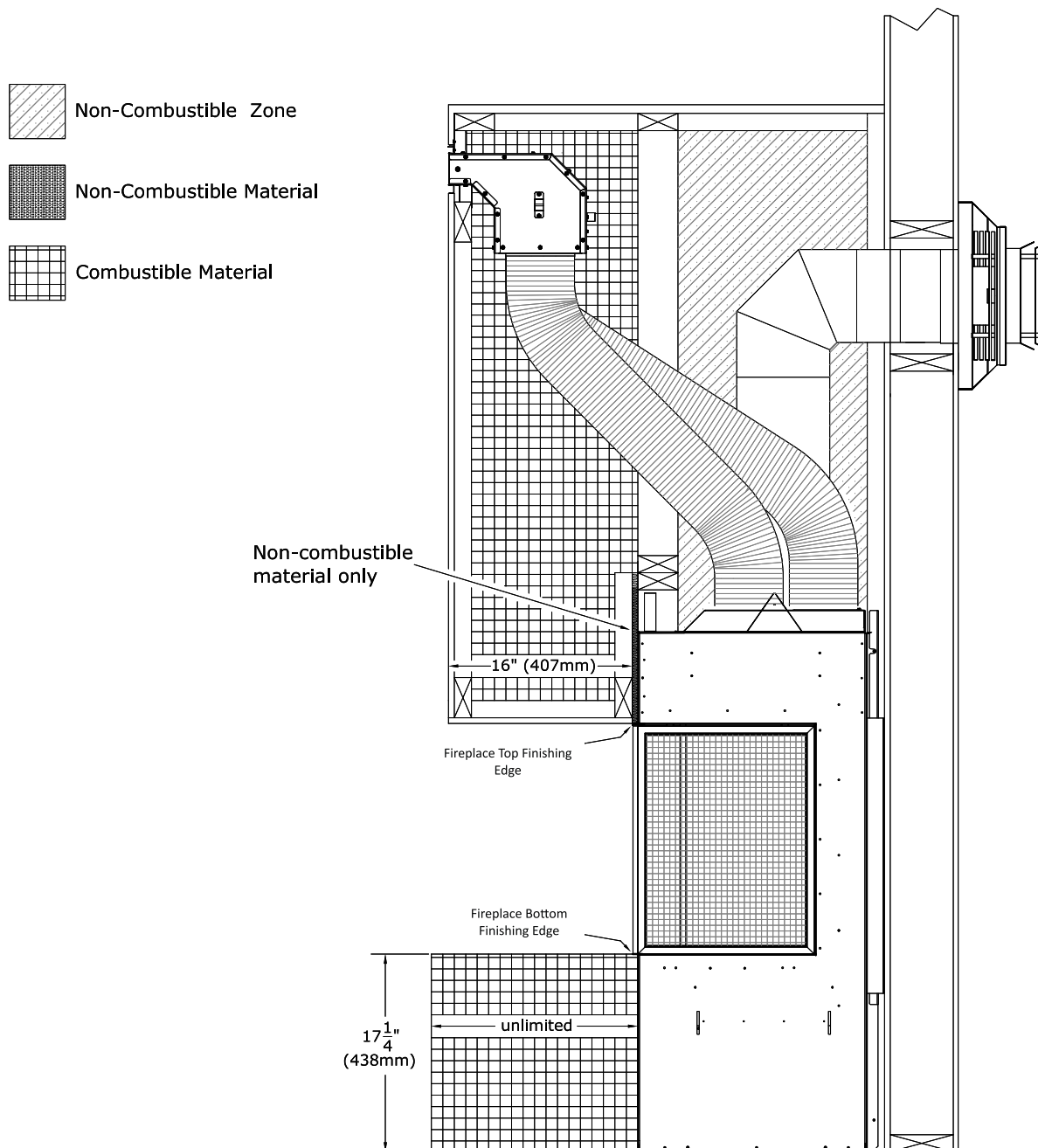
Figure 2.15 - Front Chamber Projection and Hearth Projection
