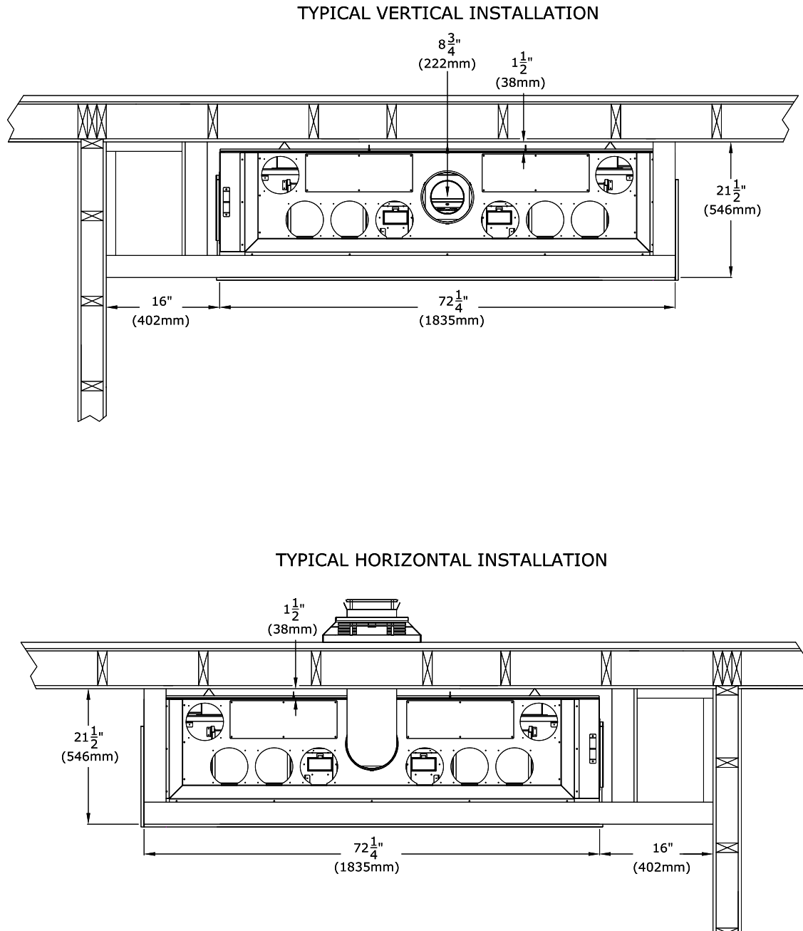
Figure 1.5 - Typical Corner Installations
