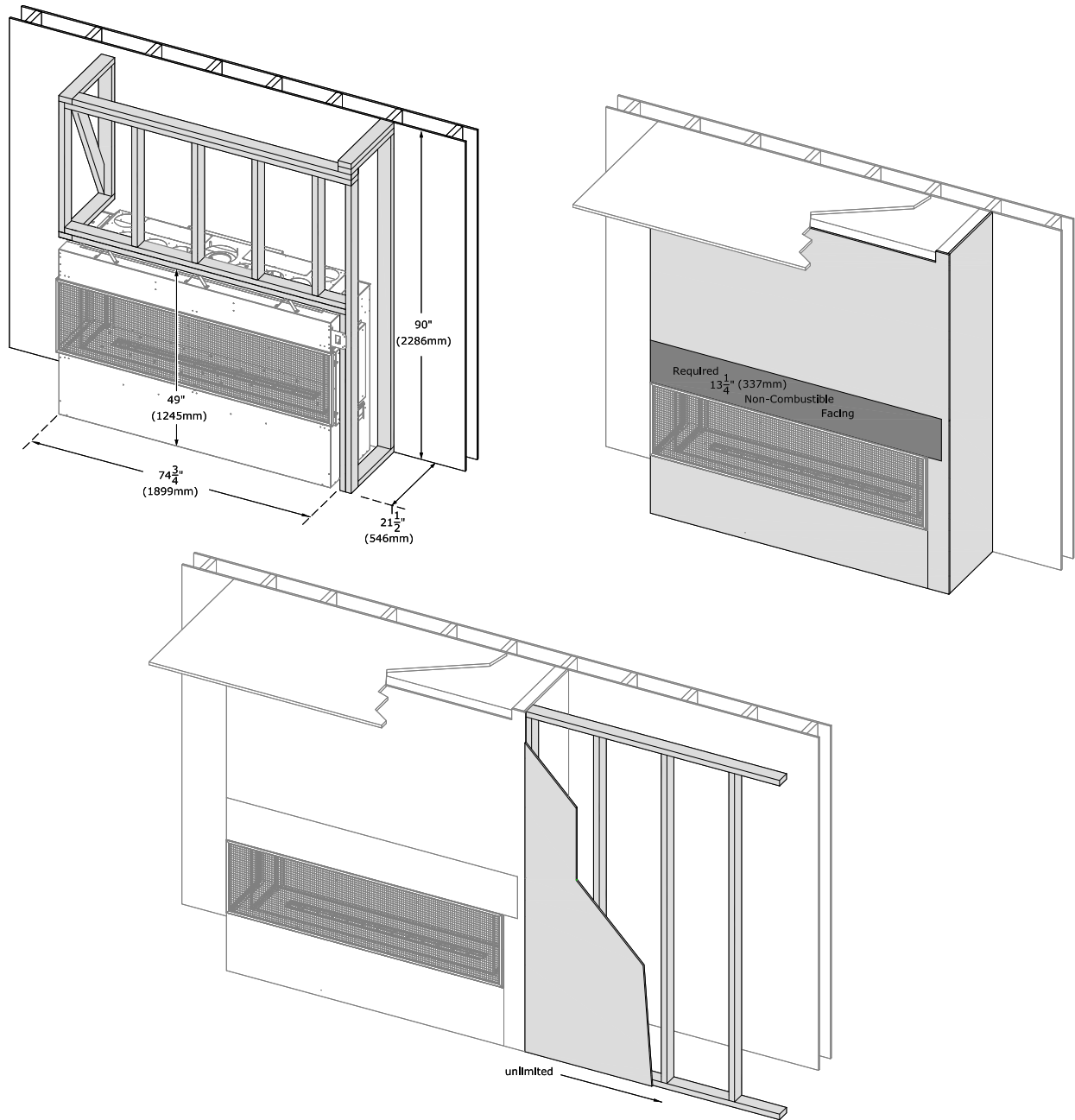
Figure 2.23 - Wall Extension - Corner Fireplace
