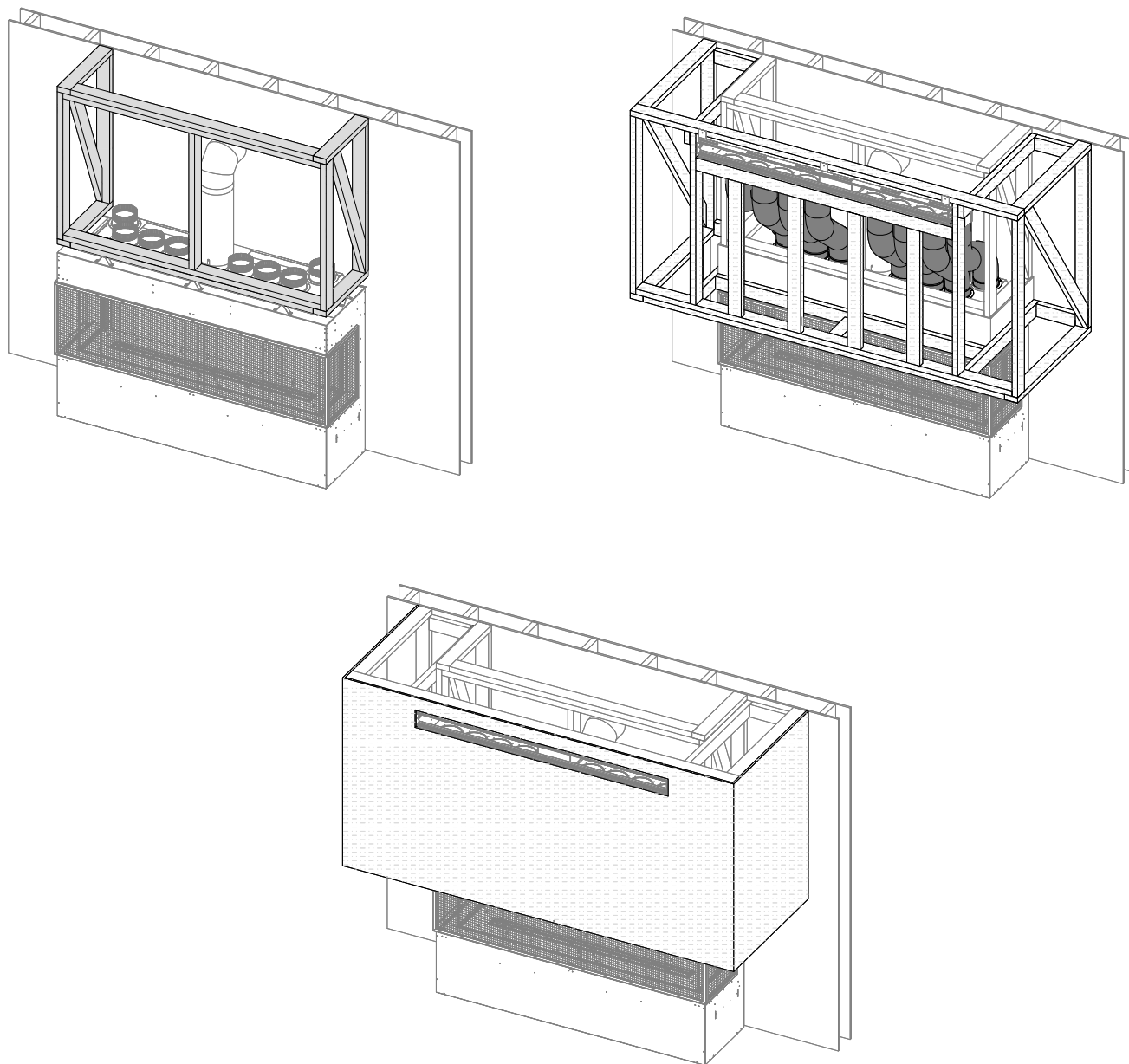
Figure 3.26 - Constructing a Chamber Projection with a KZK
