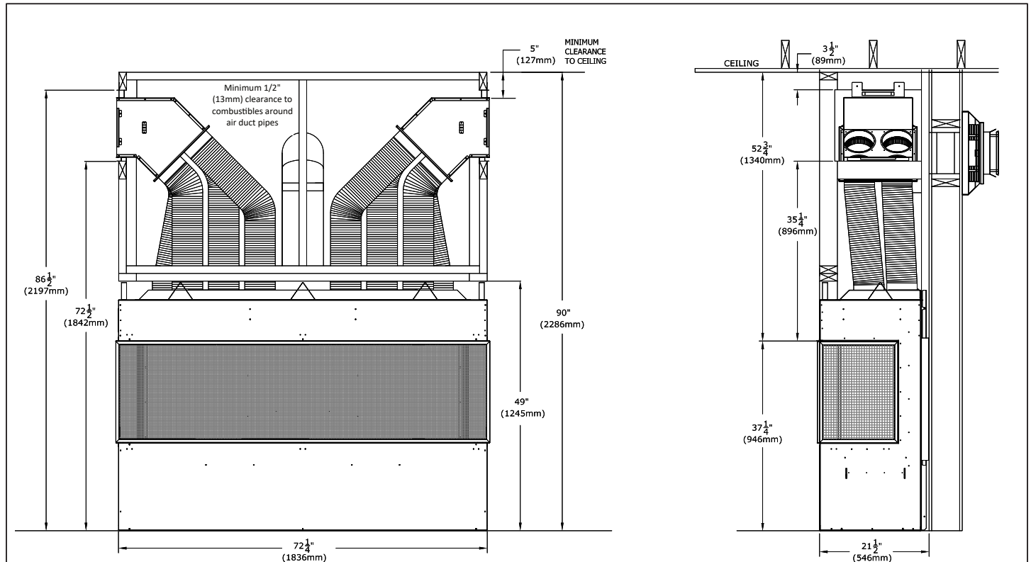
Figure 3.13- Minimum Chamber Height Plenum Framing
