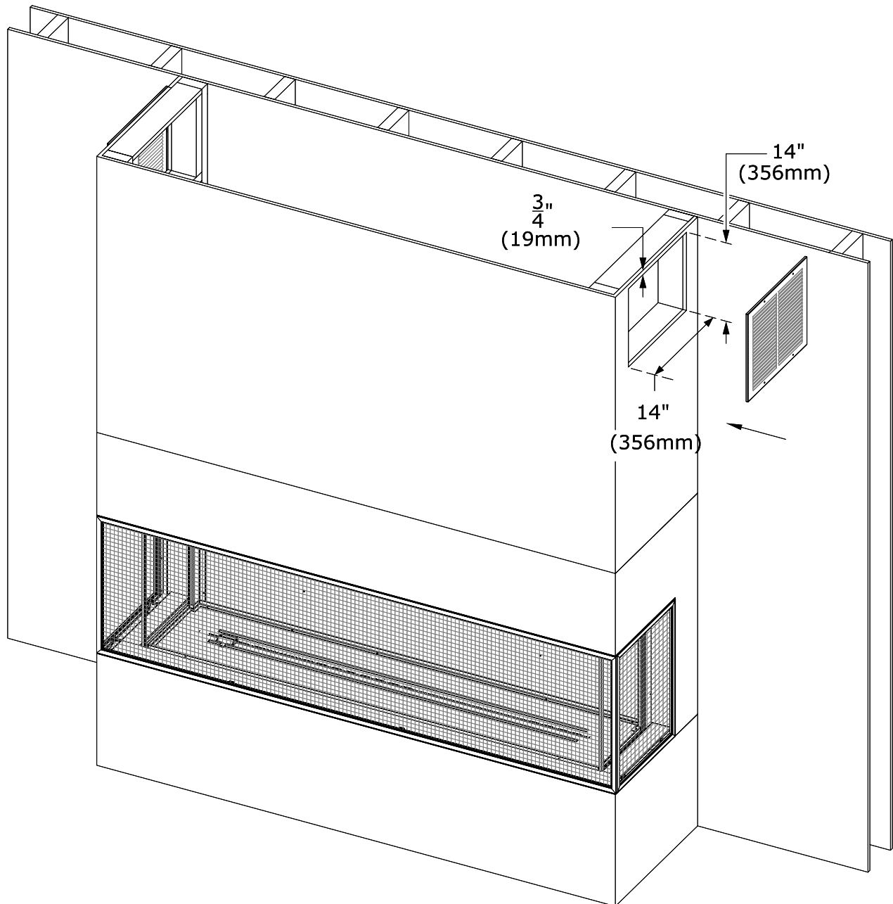
Figure 3.22 - Heat Release - Side Opening Option
