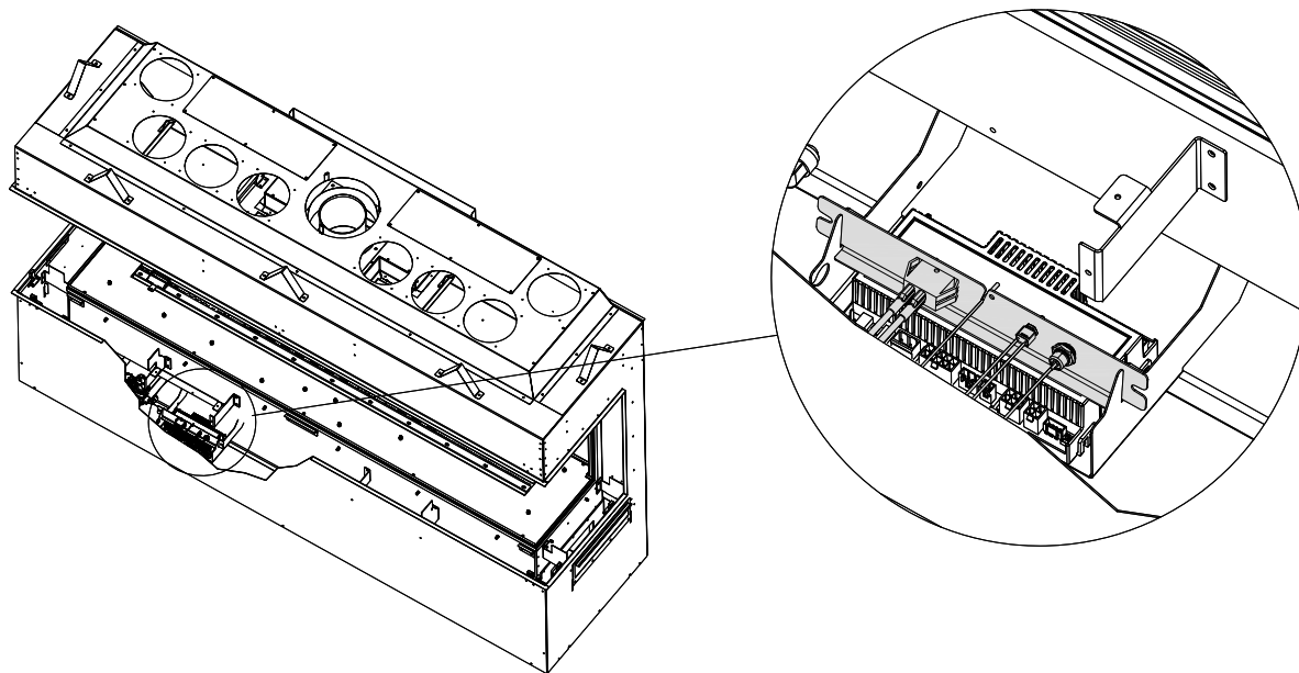
Figure 4.14 - Switch Panel Storage
