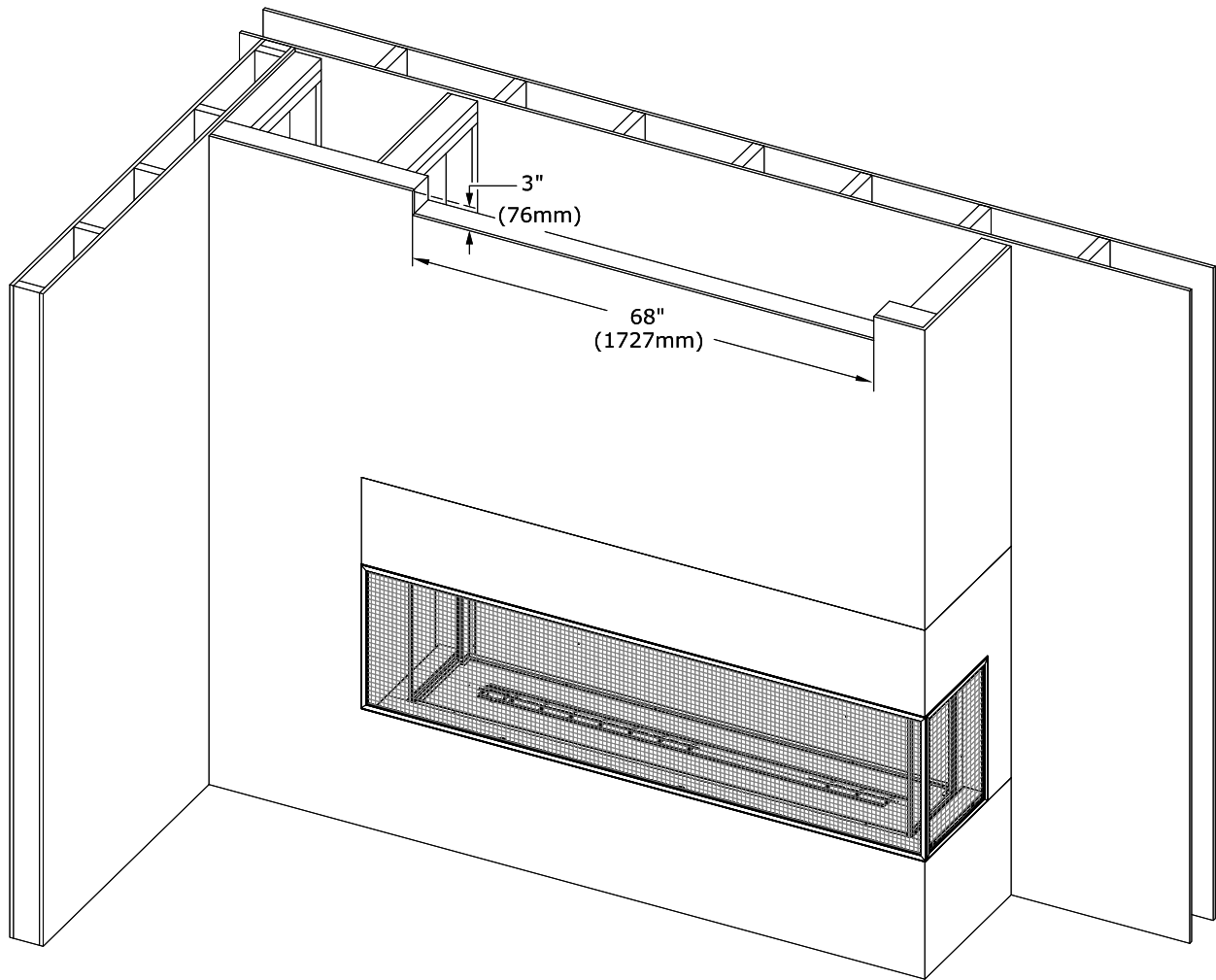
Figure 2.11 - Air Opening - Front Facing Vented Cavity
