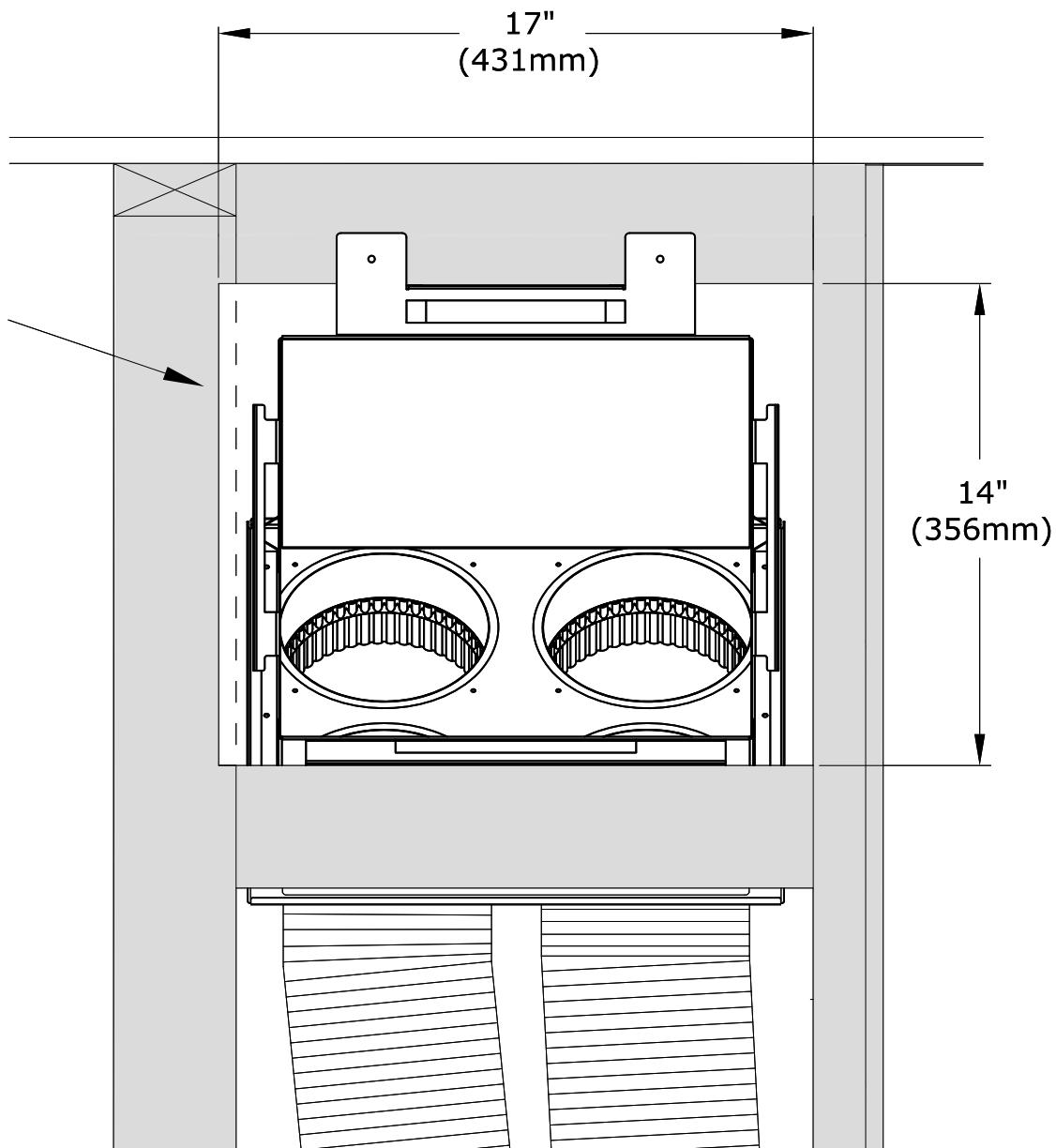
Figure 3.12 - Side KZK - Plenum Framed Opening
