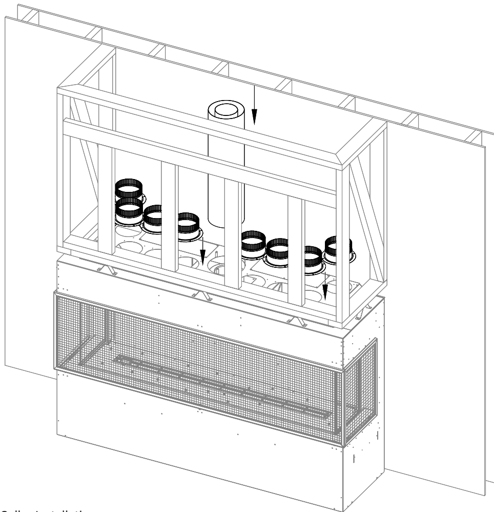
Figure 3.4 - KZK Collar Installation
