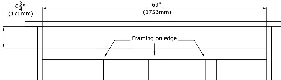
Figure 3.7 - Front KZK - Plenum Framed Opening
