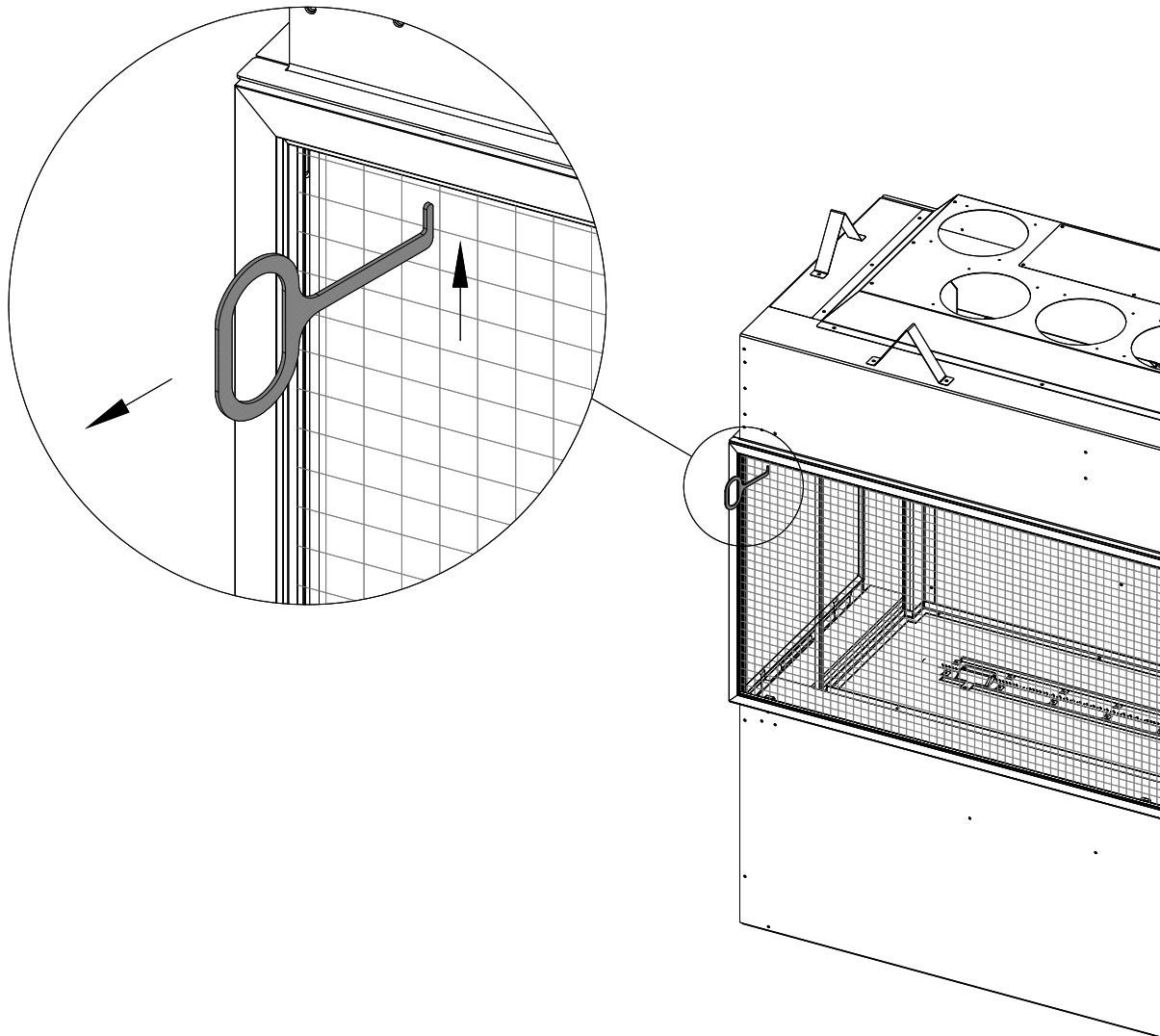
Figure 4.1 - Safety Screen Removal
