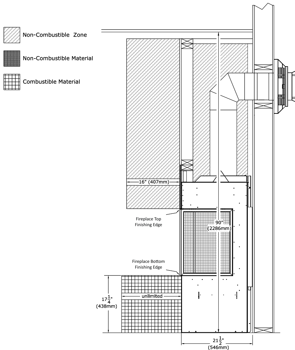
Figure 2.19 - Chamber and Hearth Projection
