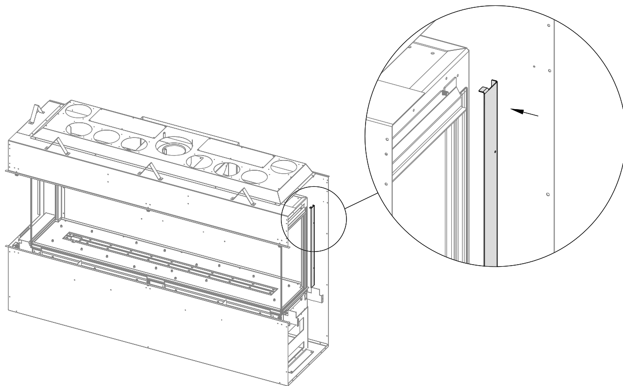
Figure 1.3 - Glass Edge Cover Installation
