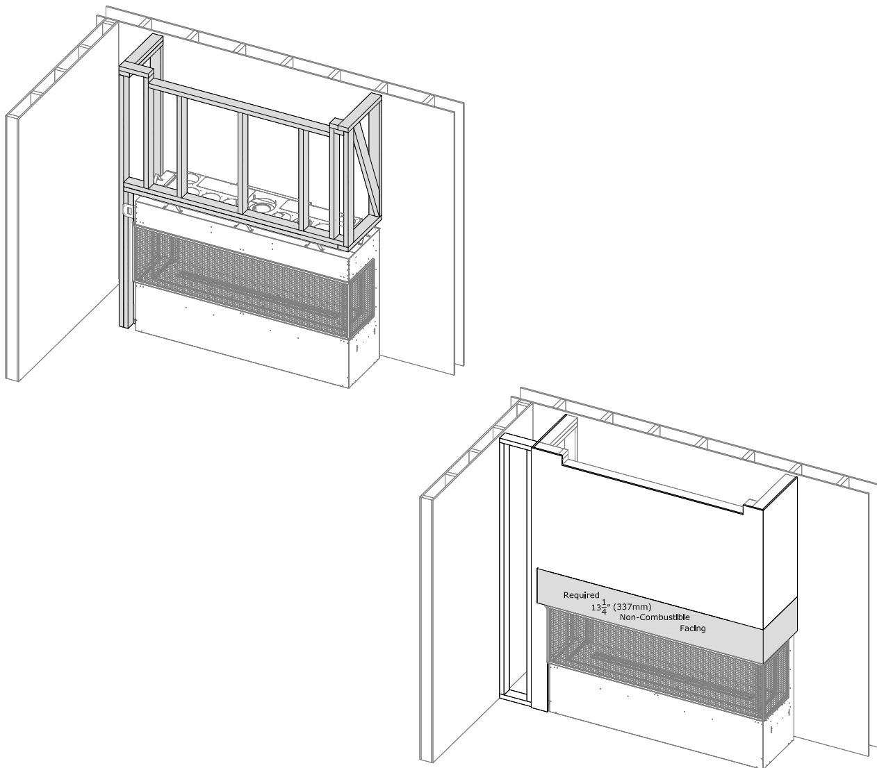
Figure 2.21 - Constructing a Chamber Projection with a Vented Cavity
