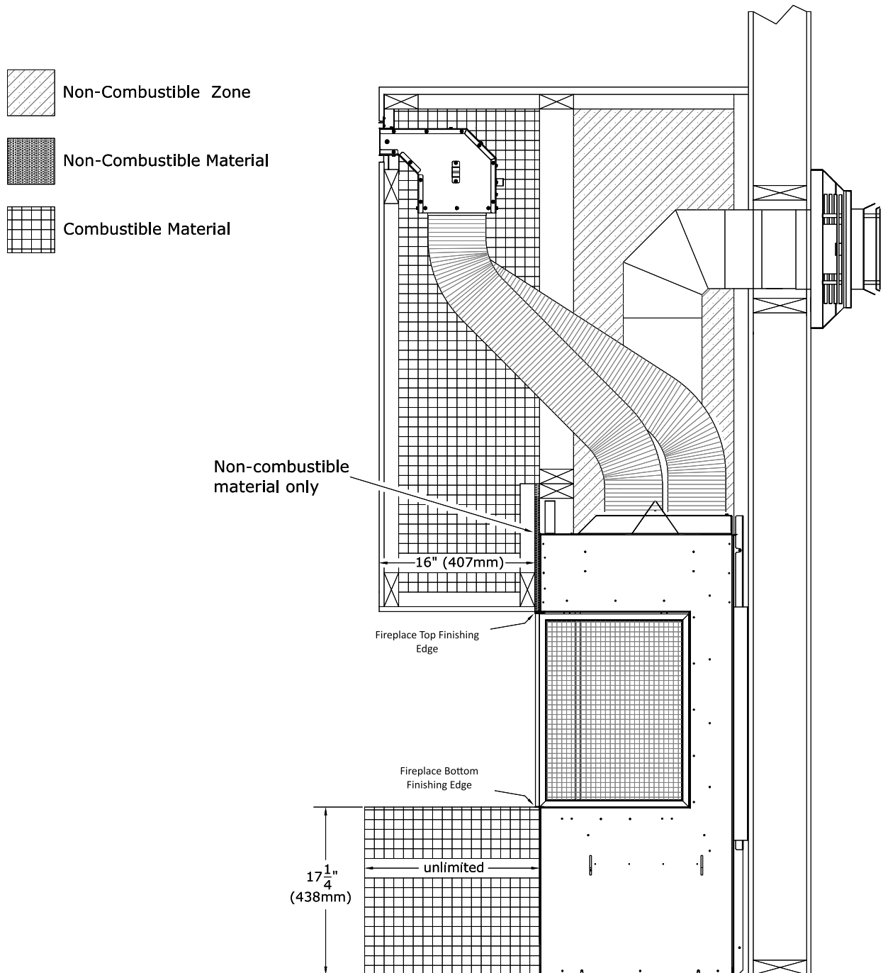
Figure 3.24 - Front Chamber Projection and Hearth Projection
