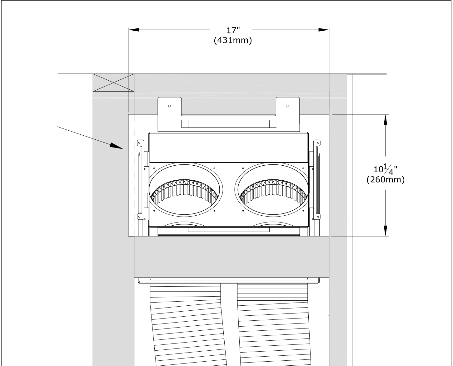
Figure 3.16 - Side KZK - Plenum Framed Opening
