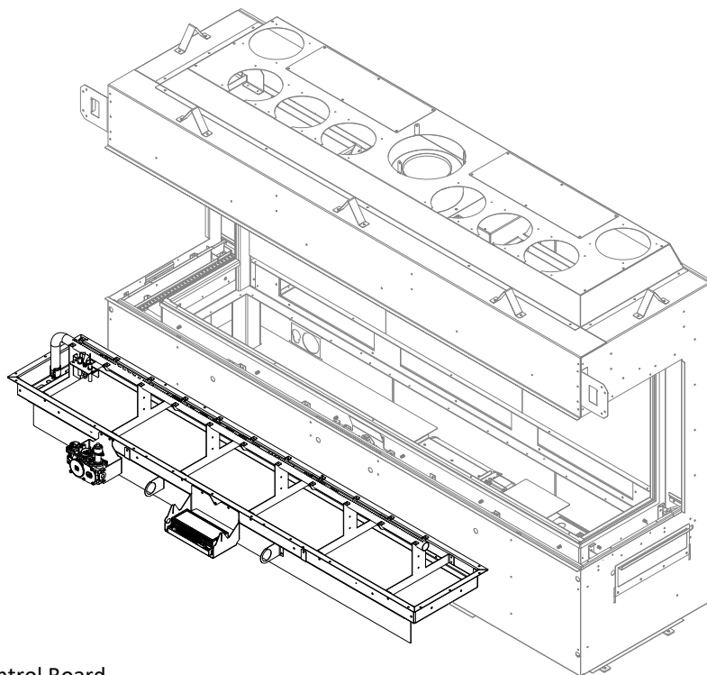
Figure 4.20 - Remove Control Board
