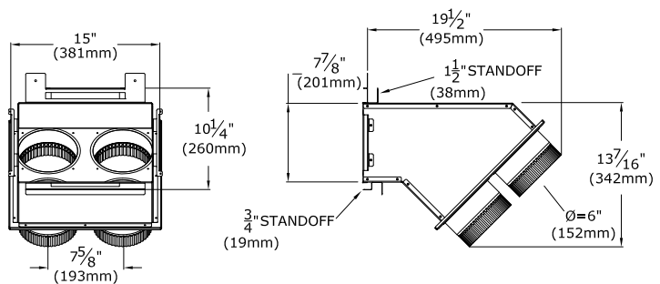
Figure 3.15 - KZK-1510B Overview
