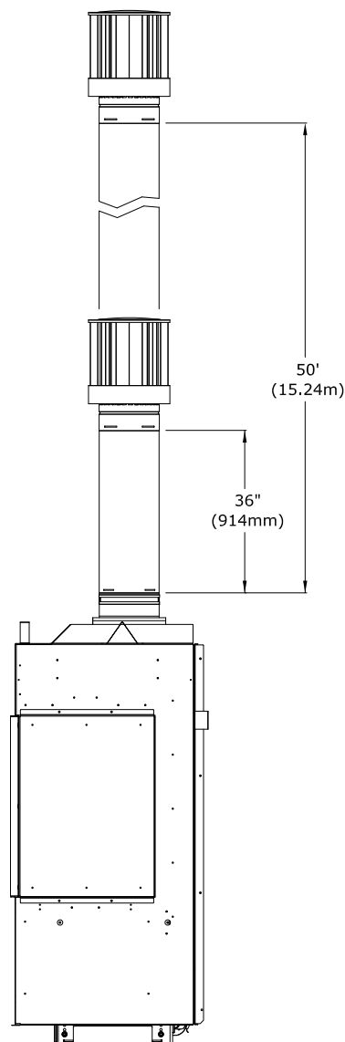
Figure 6.6 - Terminaison verticale 4 po x 6-5/8 po
