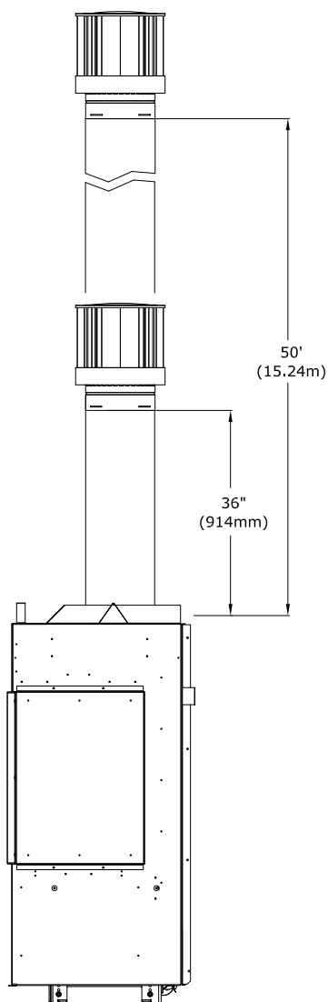
Figure 6.5 - Terminaison verticale 5 po x 8 po
