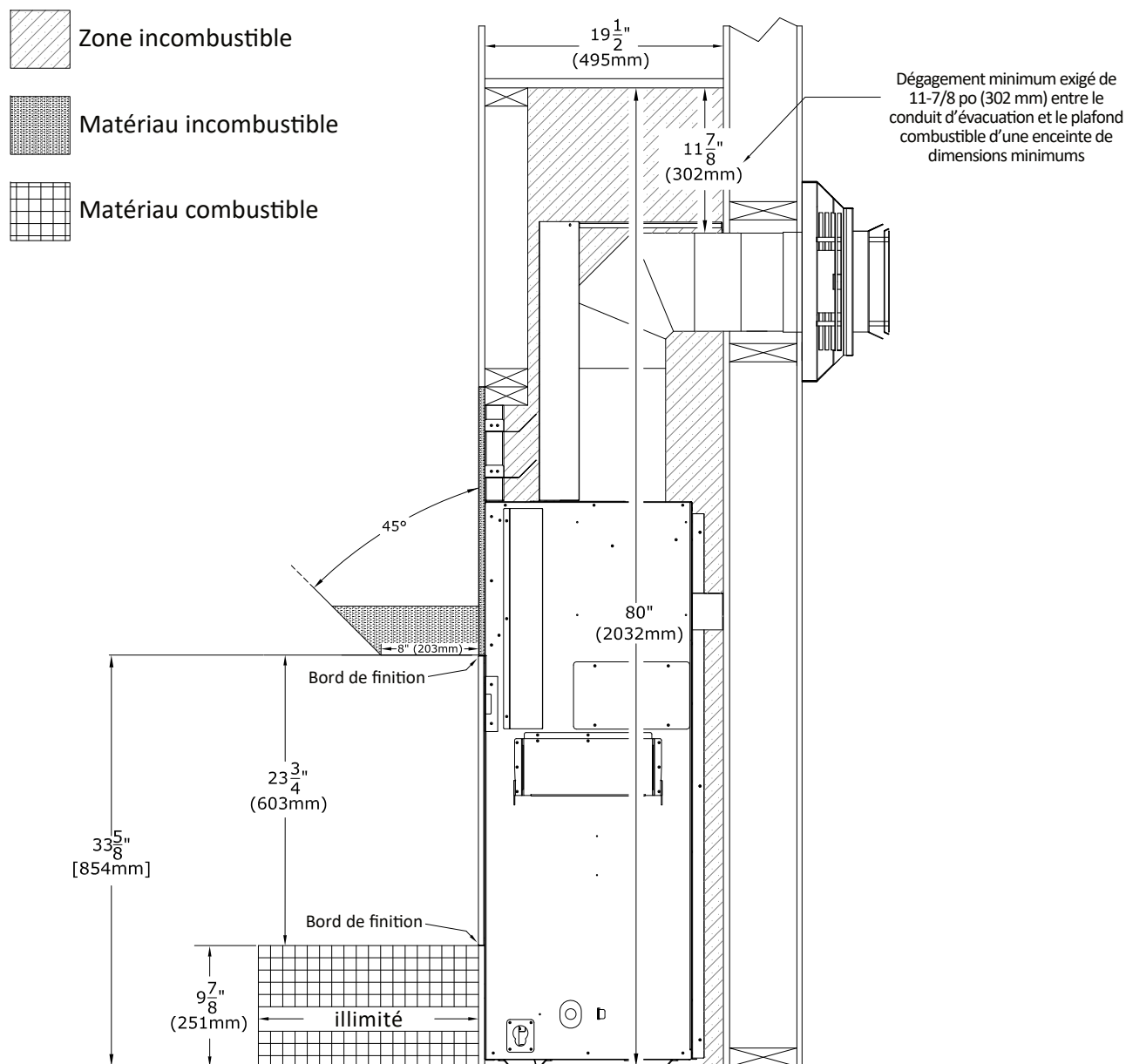
Figure 5.4 - Projections du manteau incombustible - Installation standard
