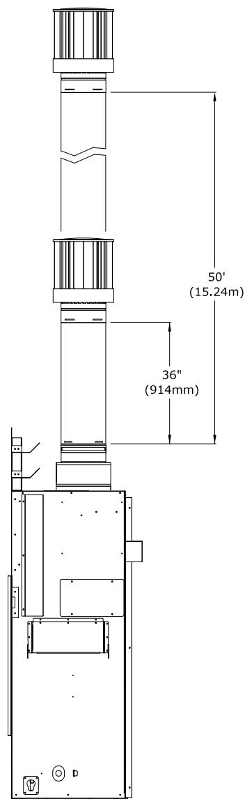
Figure 7.5 - Conduit vertical 4 po x 6-5/8 po
