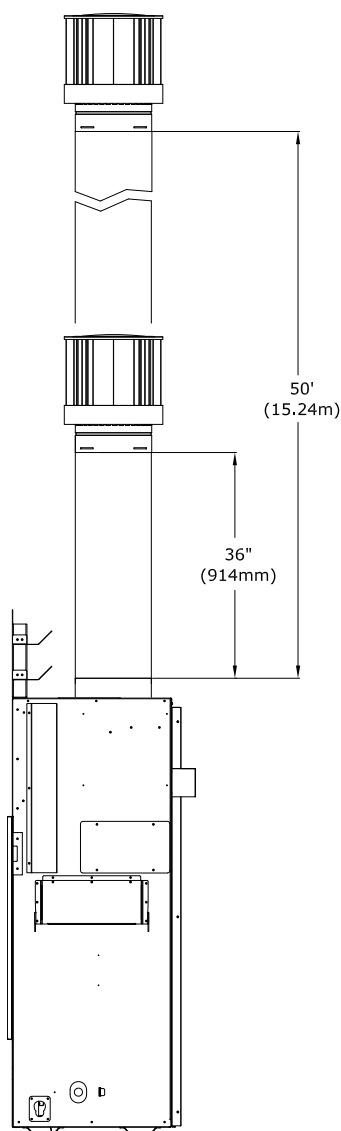
Figure 7.4 - Conduit vertical 5 po x 8 po
