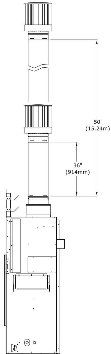
Figure 7.5 - 4"x6-5/8" Vertical Vent Pipe
