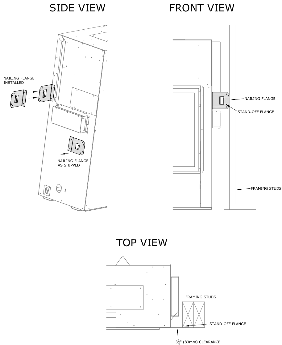
Figure 3.3 - Nailing Flange Installation
