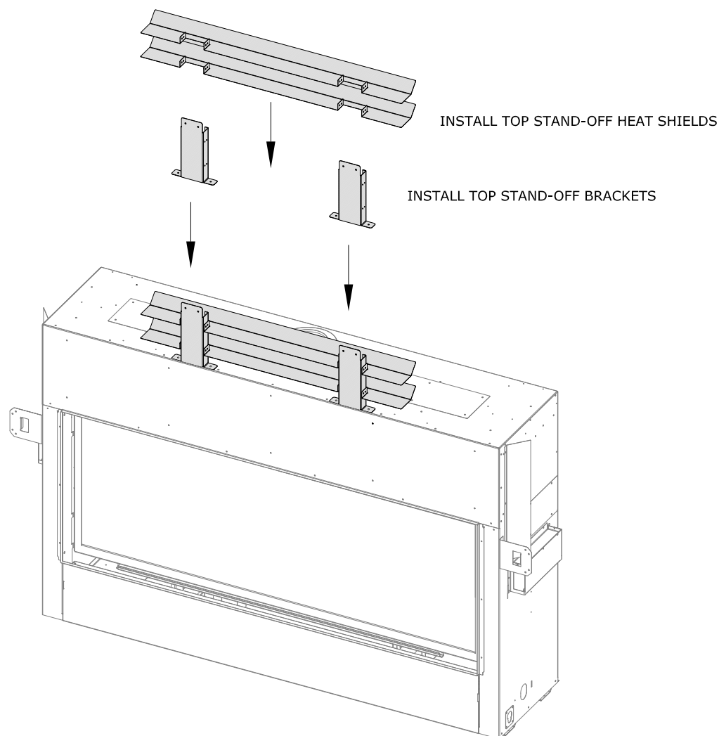
Figure 3.2 - Stand-Off Installation
