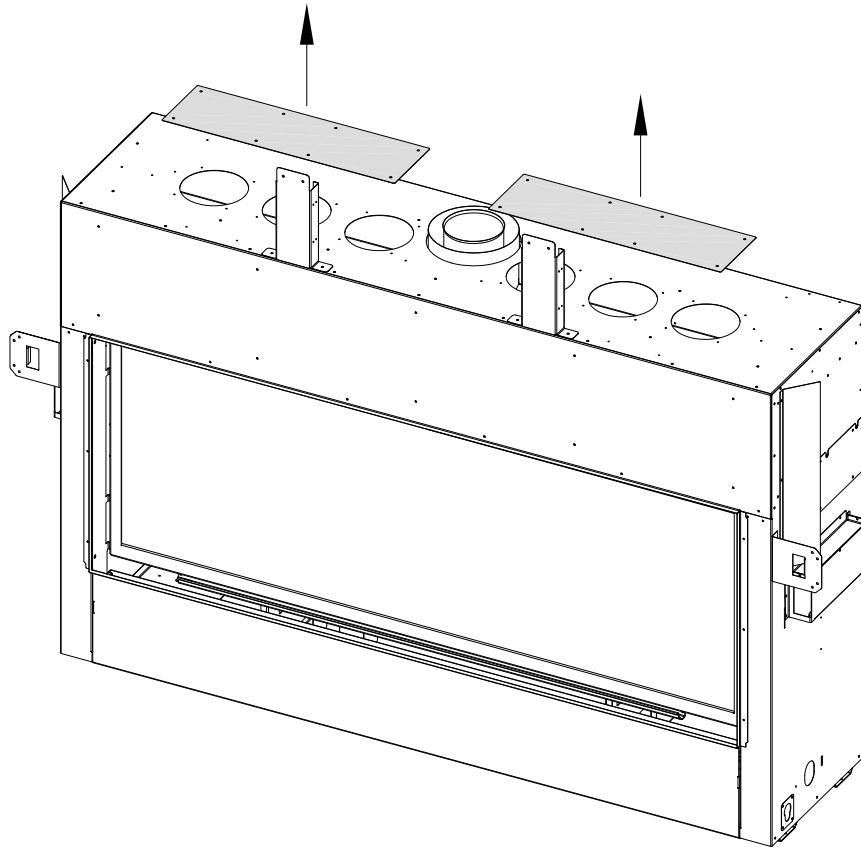
Figure 4.1 - Cover Plate Removal
