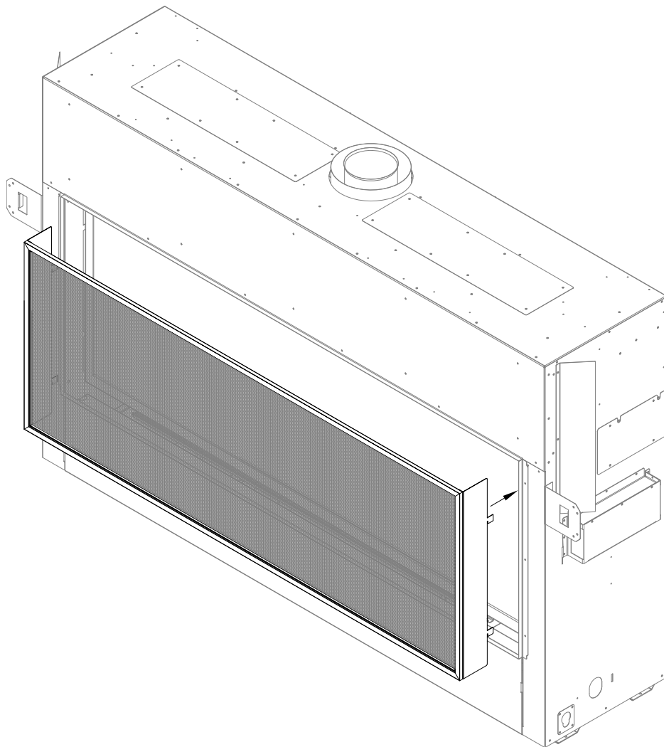
Figure 8.6 - Safety Screen Installation
