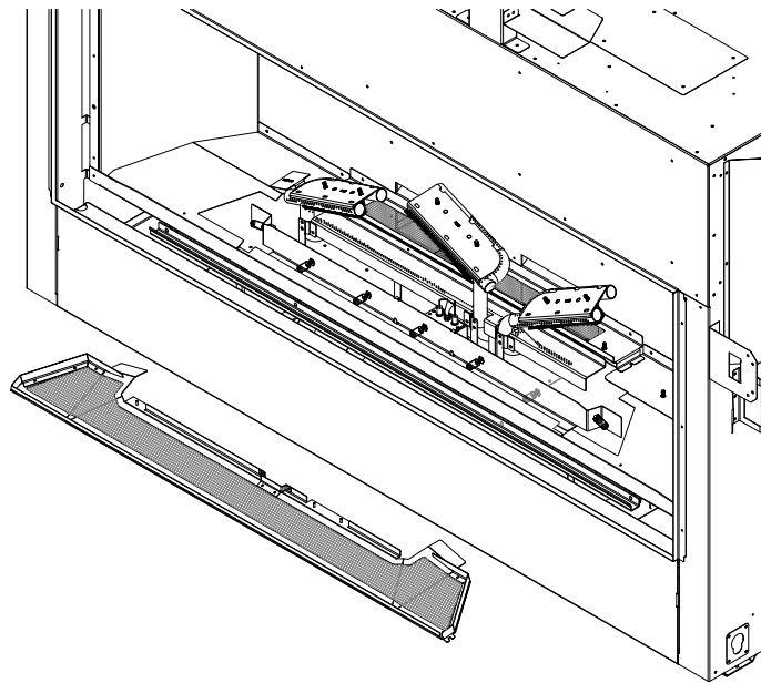
Figure 8.3 - Ember Media Tray Removal
