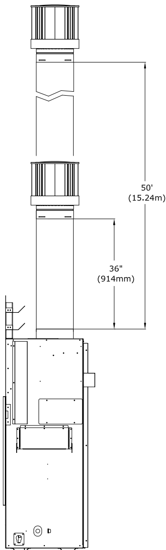
Figure 7.4 - 5"x8" Vertical Vent Pipe
