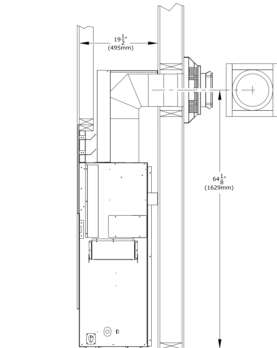
Figure 3.8 - Minimum Wall Thimble Framing
