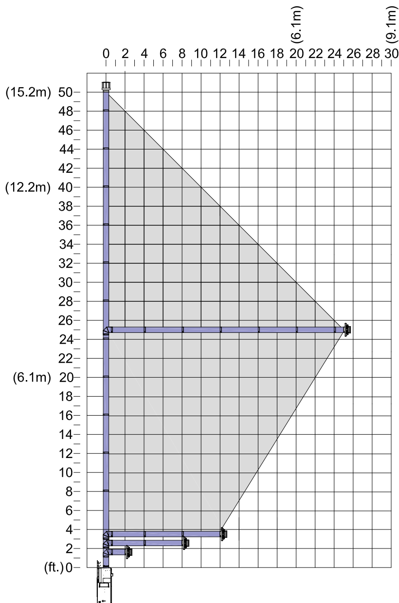
Figure 7.8 - Combination Venting
