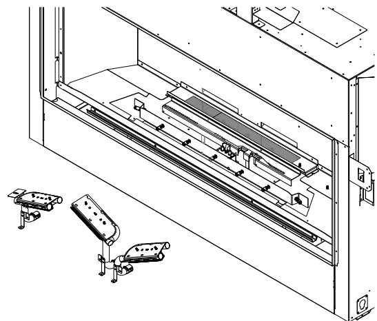
Figure 8.10 - Step 3
