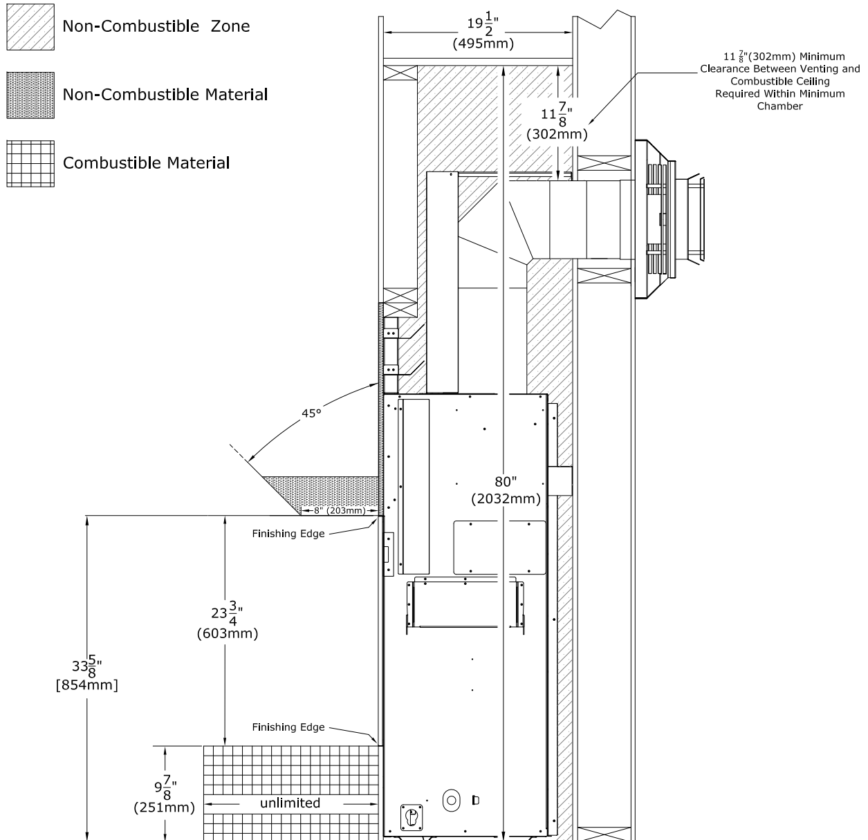
Figure 5.4 - Non-Combustible Mantel Projection - Standard Installation
