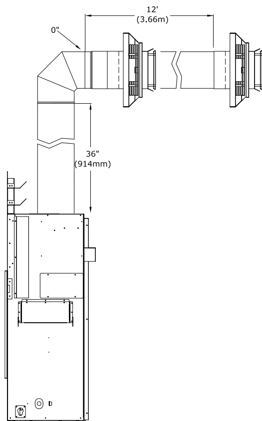
Figure 7.7 - Horizontal 5'x8" Terminations
