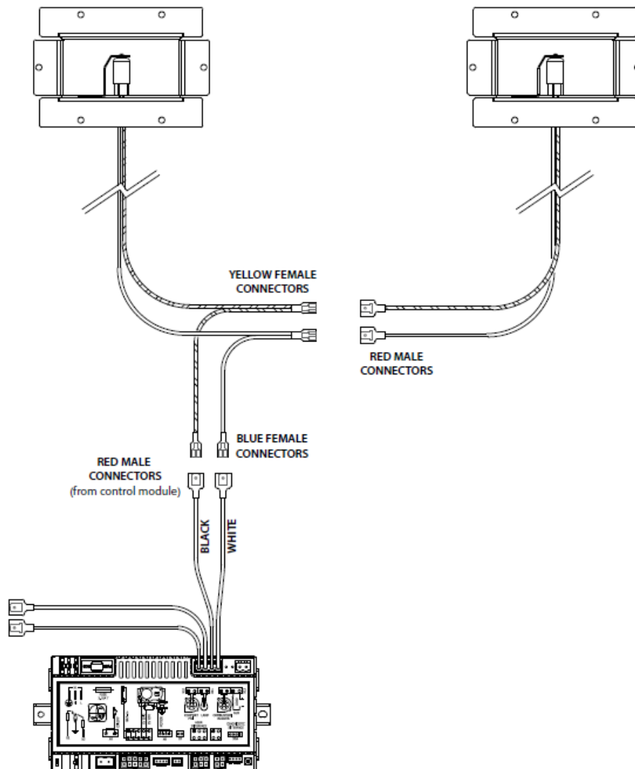
Figure 8.14 - Top Light Kit Wiring
