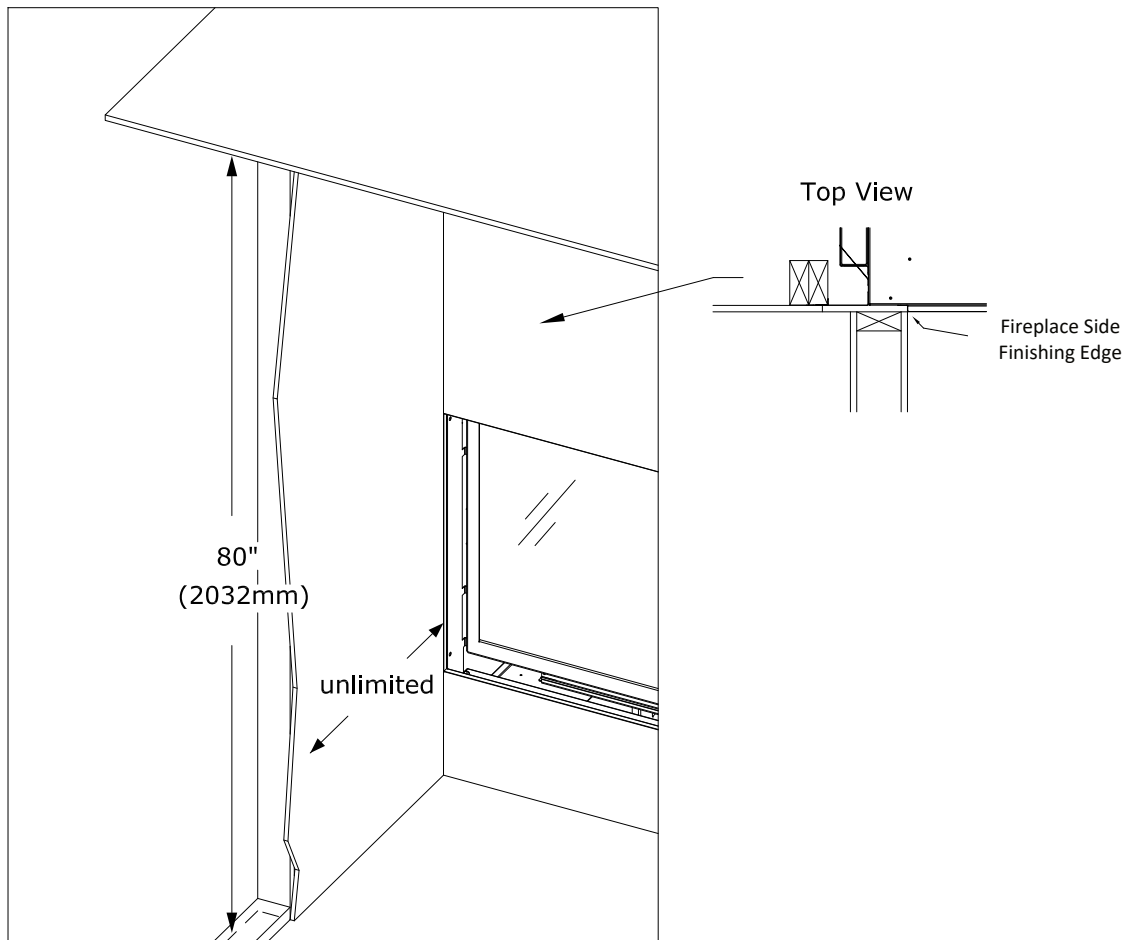
Figure 5.3 - Combustible Sidewall Projection
