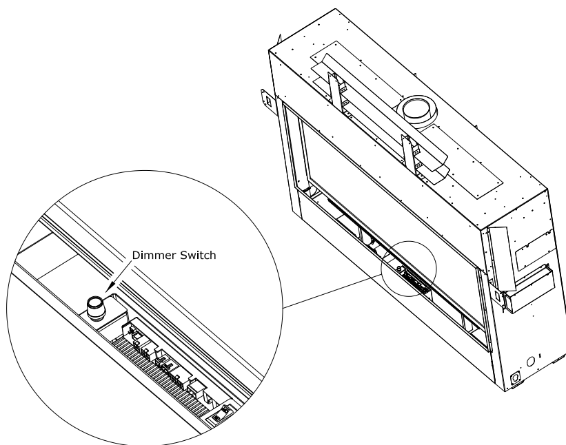
Figure 10.15 - Ember Bed Dimmer Switch
