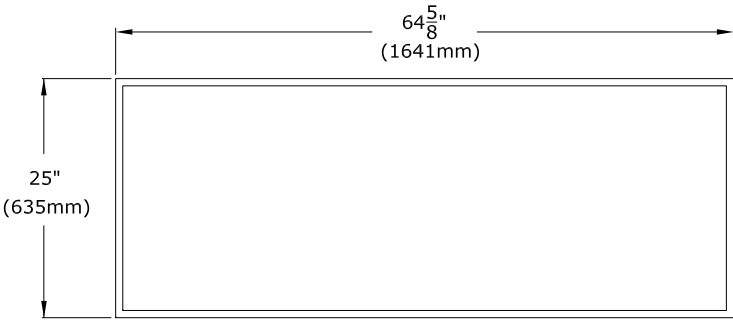
Figure 2.4 - Optional Surround Dimensions Rectangle Surround NK60TL-RS
