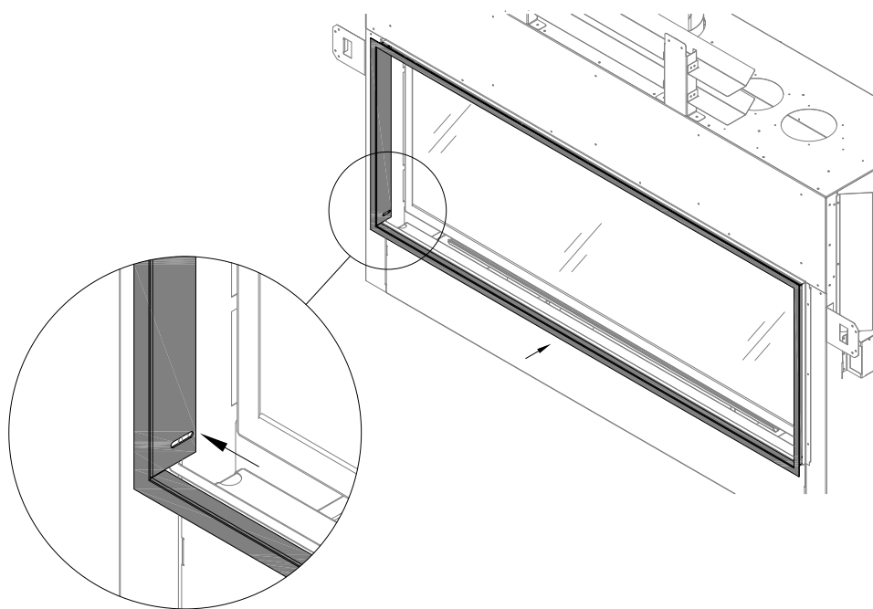
Figure 8.7 - Rectangle Surround Installation
