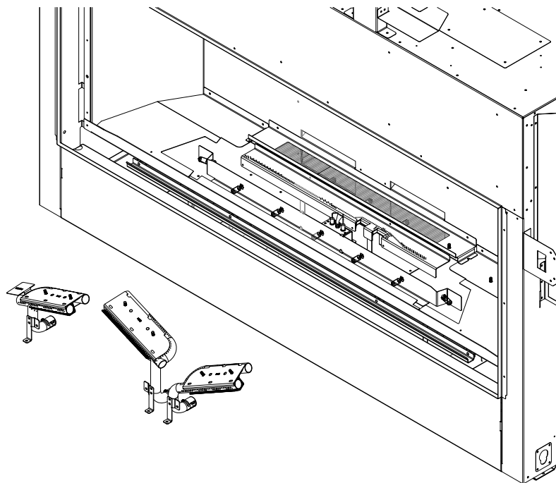
Figure 8.4 - Left, Center, and Right Burner Removal
