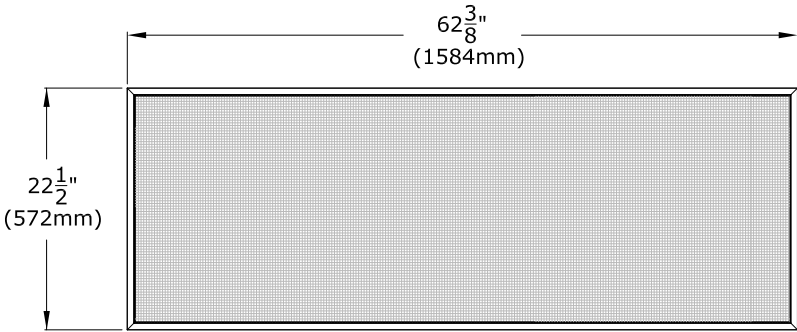
Figure 2.3 - Safety Screen Barrier Dimensions Safety Screen Barrier NK60TL-ES
