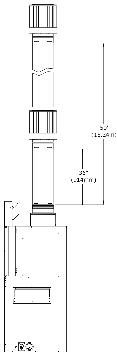
Figure 8.4 - Conduit vertical 4 po x 6-5/8 po
