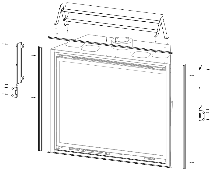
Figure 5.6 - Installation du kit de garnitures de finition
