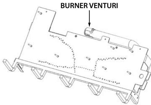
Figure 3, Burner Venturi Location
