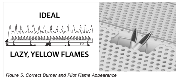
Figure 5, Correct Burner and Pilot Flame Appearance
