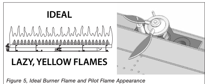
Figure 5, Ideal Burner Flame and Pilot Flame Appearance
