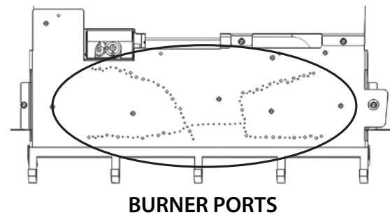
Figure 4, Burner Ports Location
