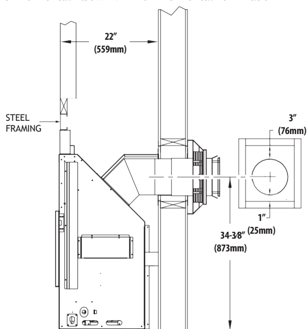
Natural Gas and Propane 45° Horizontal Elbow - Minimum Horizontal Termination
