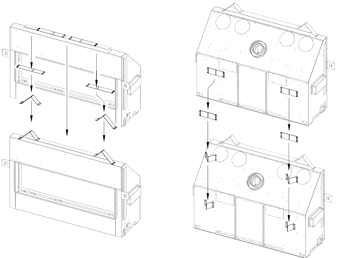
FIGURE 3.3 Stand-off Assembly and Installation
