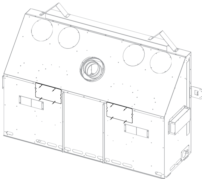
FIGURE 3.10 Heat Transfer Kit Cover Plate Removal
