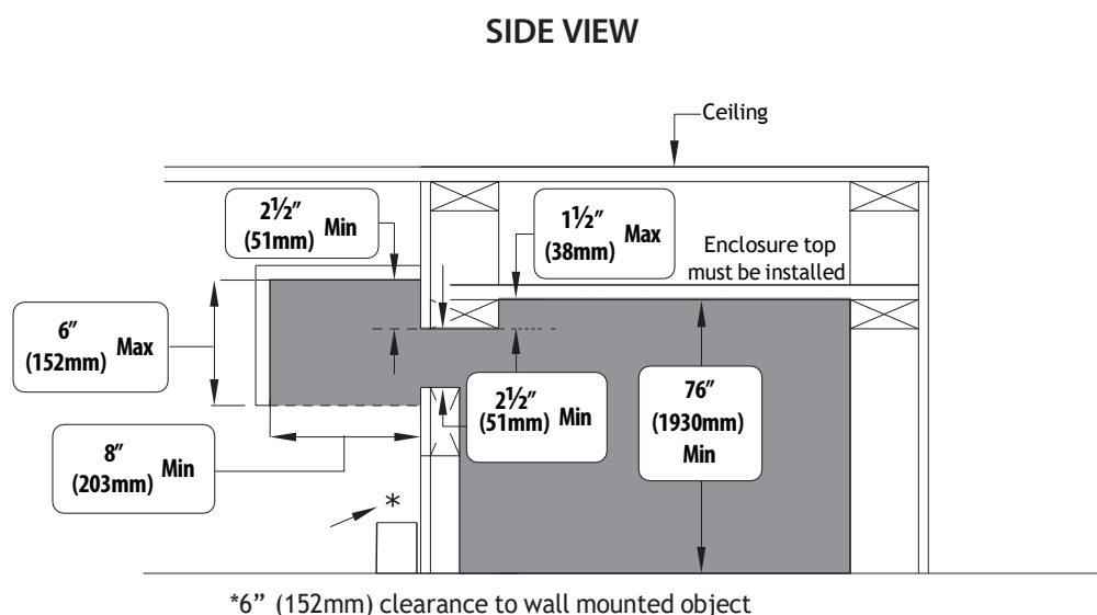
FIGURE 3.18 Lowered Air Discharge Opening with Overhang
