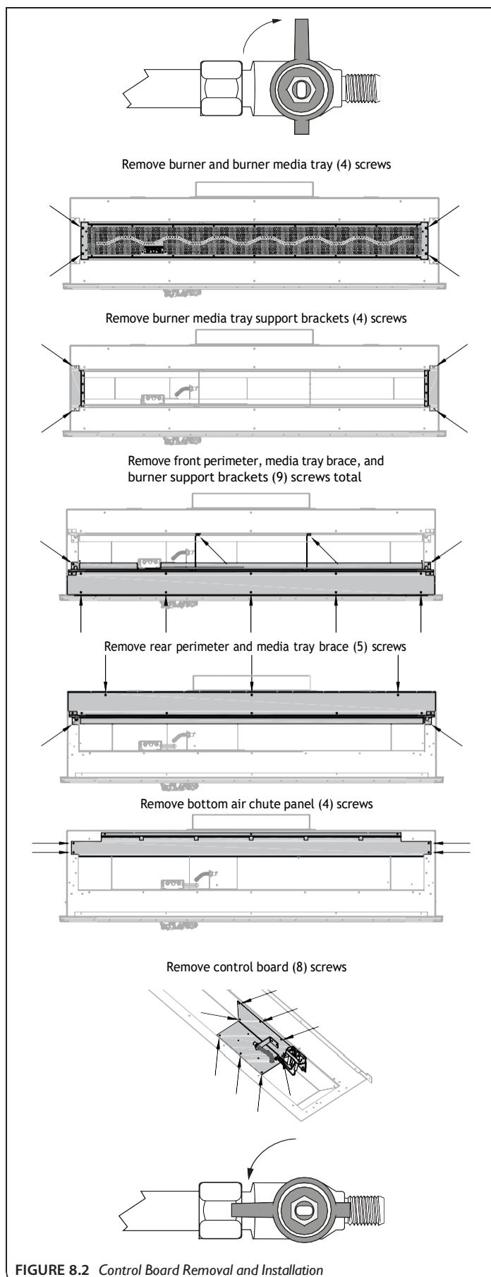
FIGURE 8.2 Control Board Removal and Installation
