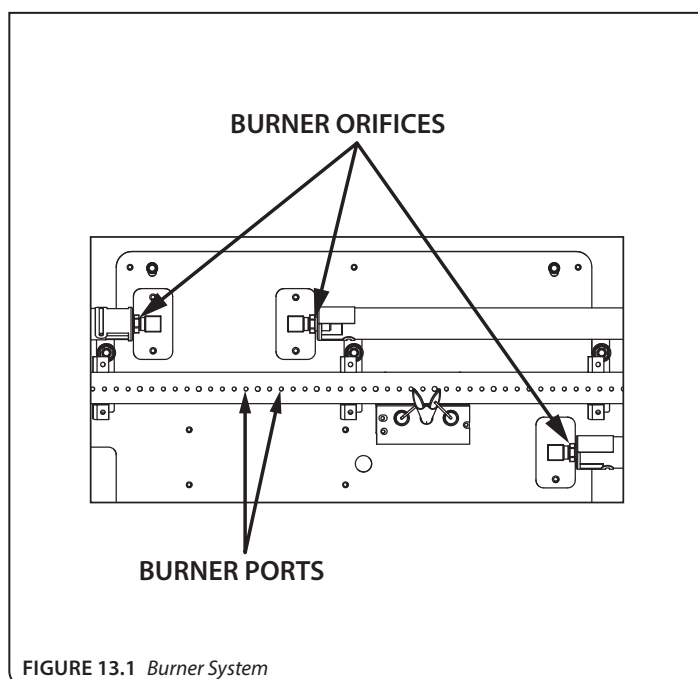
FIGURE 13.1 Burner System
