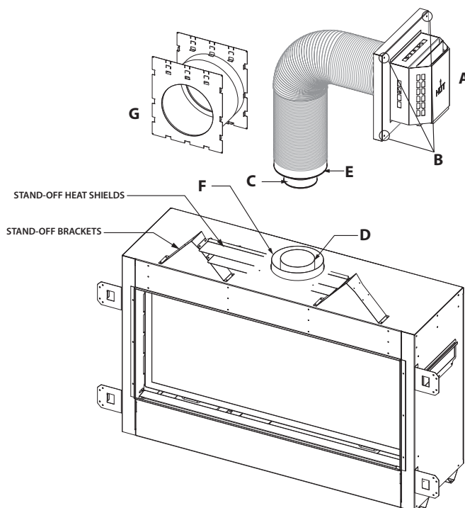
FIGURE 7.7 Installation and Assembly #800-1 Series
