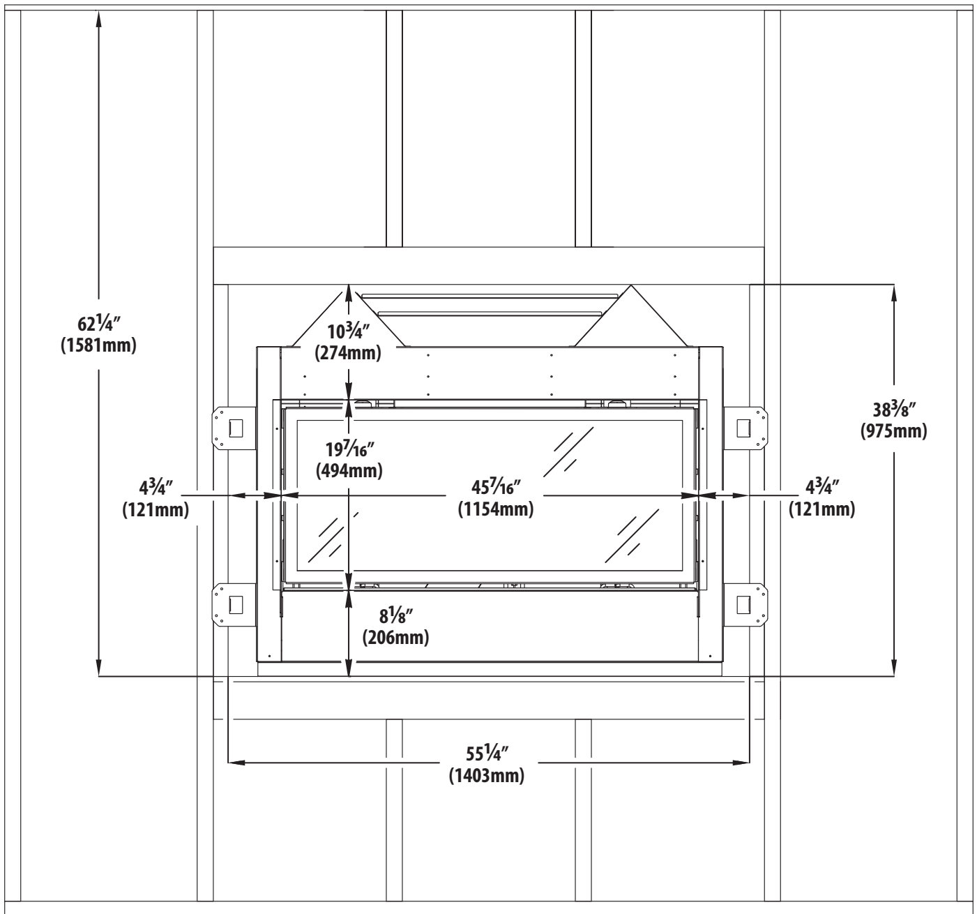
Nominal 2" x 4" framing used in enclosure framing
