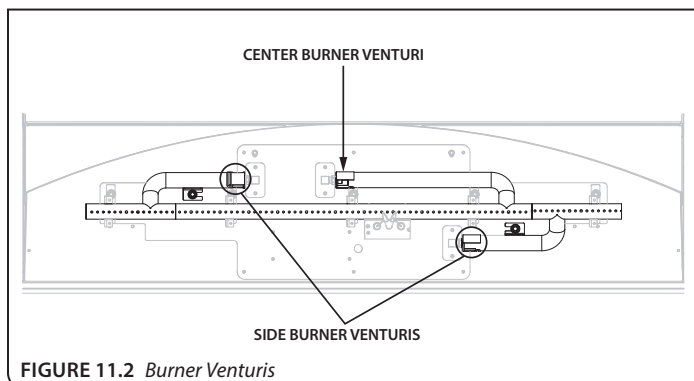
FIGURE 11.2 Burner Venturis
