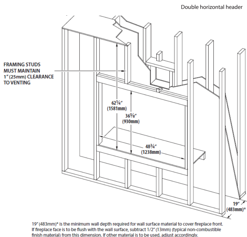
Nominal 2" x 4" framing used in enclosure framing
