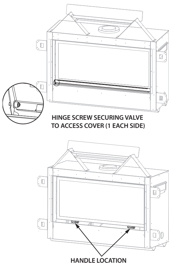
FIGURE 8.1 Glass Frame Assembly Removal and Installation
