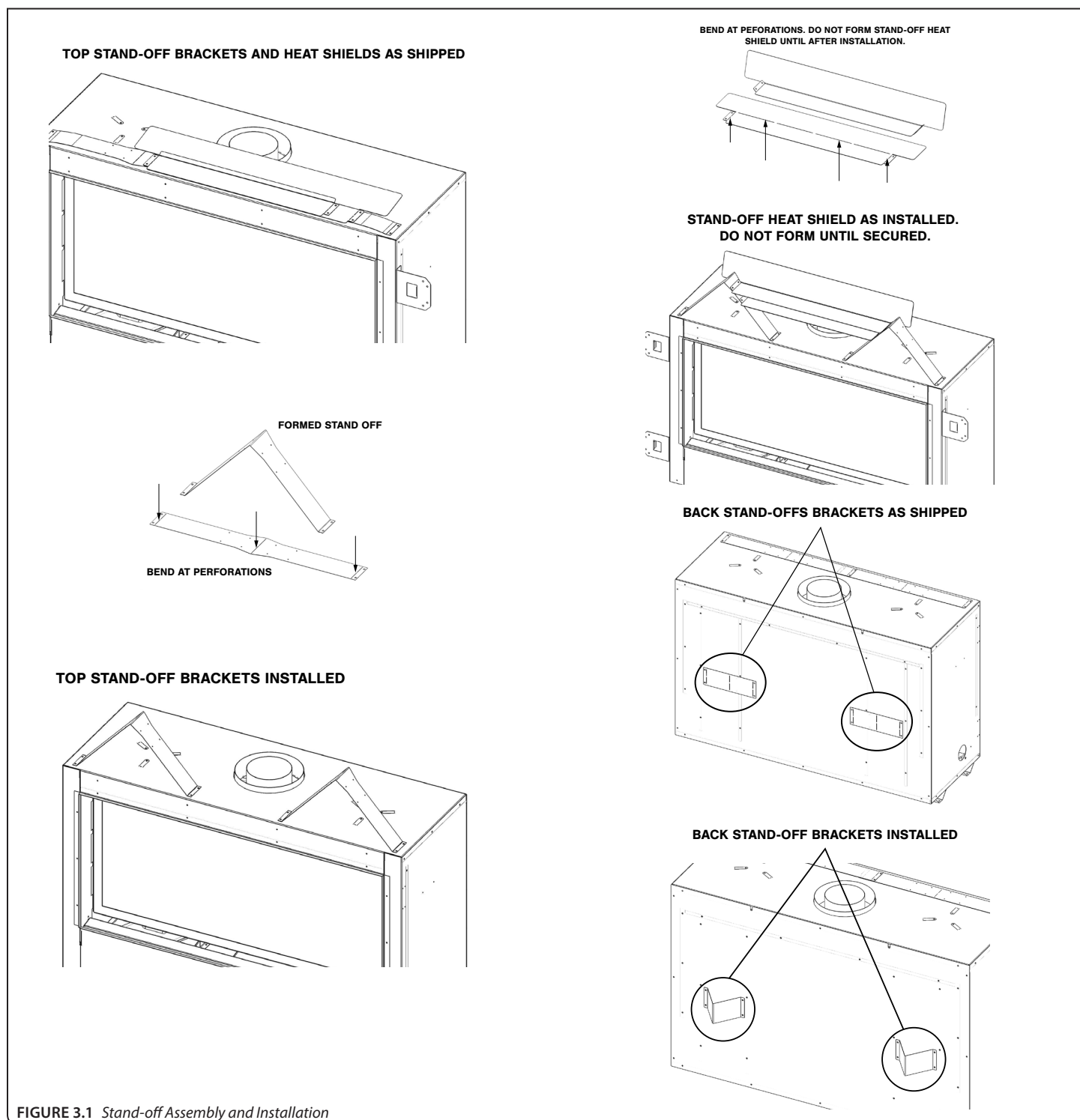
FIGURE 3.1 Stand-off Assembly and Installation
