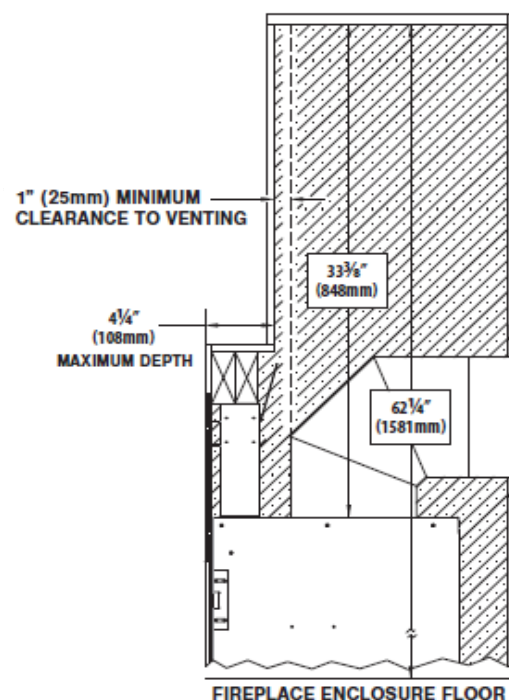
TV Recess Construction
