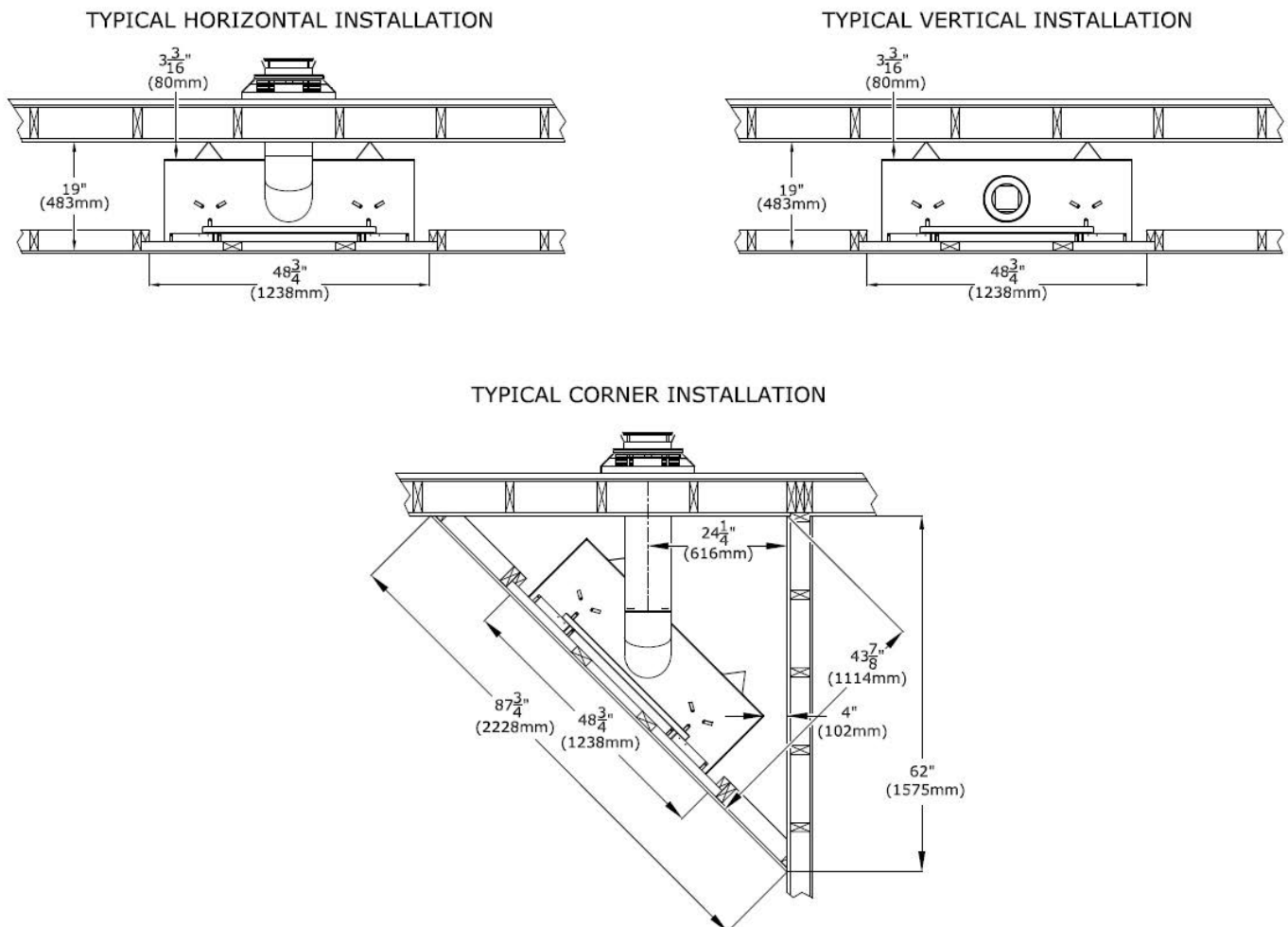
FIGURE 3.3 Typical Install Options
