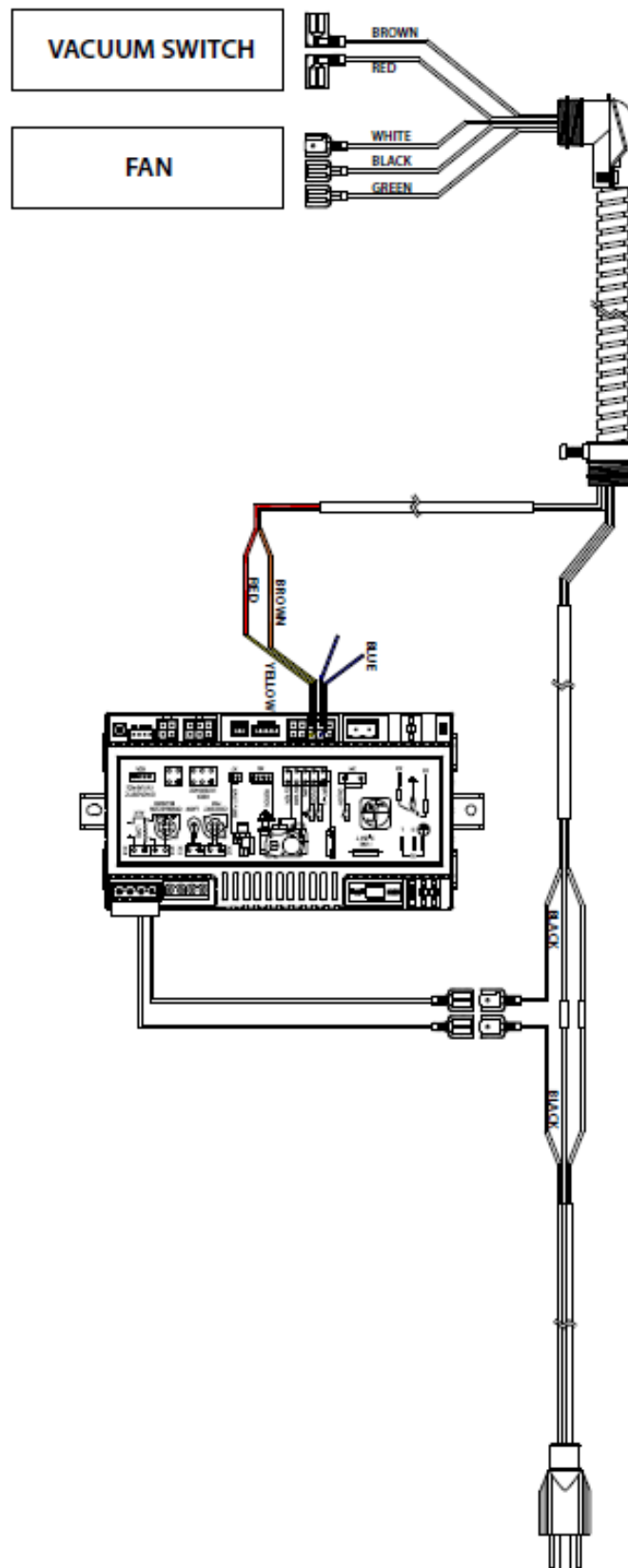
Figure 7.4 - Electrical Diagram
