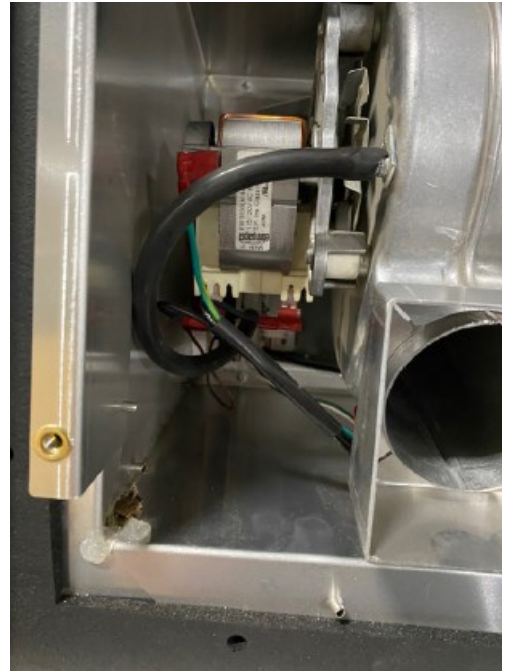
Figure 8.8 - Screws Securing Vacuum Switch Bracket
