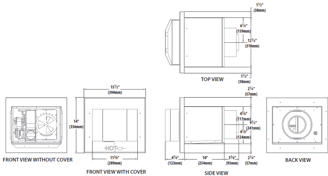
Figure 1.1 - #KPV Dimensions
